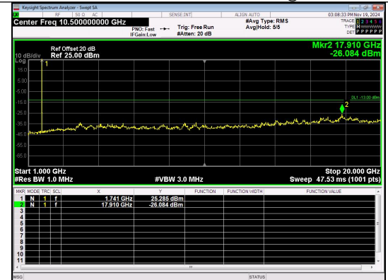
1000.0MHz-20000.0MHz Band 66 5MHz/1745.0/Mid 16QAM 1@0
