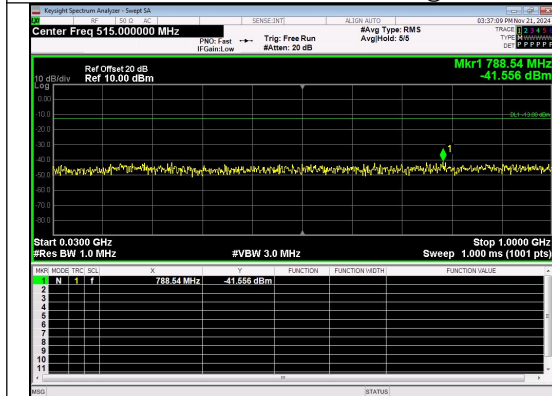
30.0MHz-1000.0MHz Band 66 10MHz/1715.0/Low 16QAM 1@0
