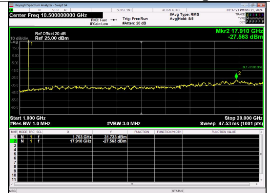
1000.0MHz-20000.0MHz Band 66 10MHz/1715.0/Low 16QAM 1@0
