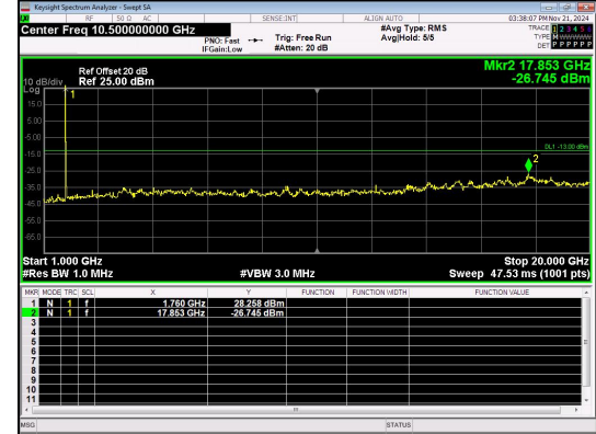
1000.0MHz-20000.0MHz Band 66 15MHz/1772.5/High 16QAM 1@0
