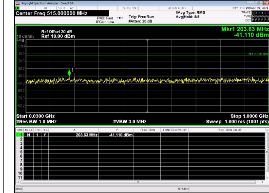
30.0MHz-1000.0MHz Band 66 10MHz/1745.0/Mid 16QAM 1@0
