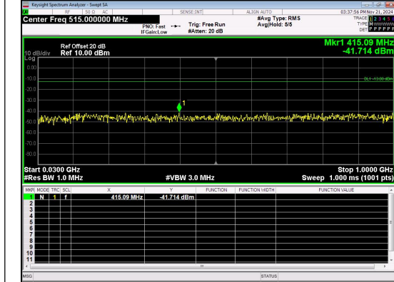
30.0MHz-1000.0MHz Band 66 15MHz/1772.5/High 16QAM 1@0
