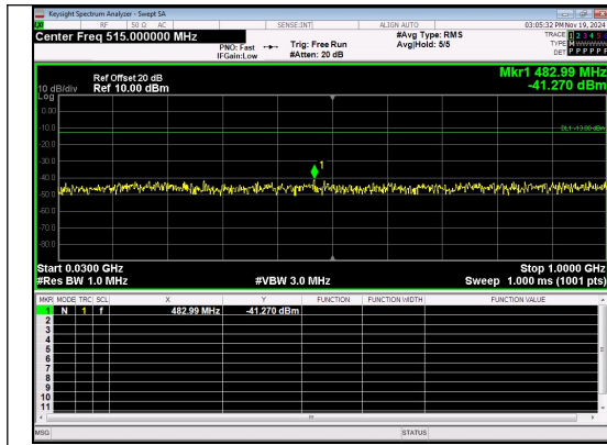
30.0MHz-1000.0MHz Band 66 5MHz/1777.5/High QPSK 1@0
