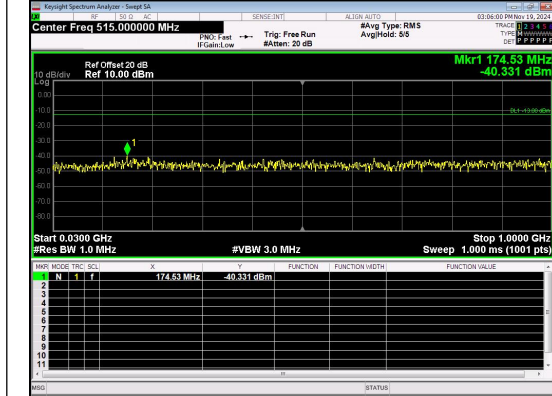
30.0MHz-1000.0MHz Band 66 5MHz/1777.5/High 16QAM 1@0
