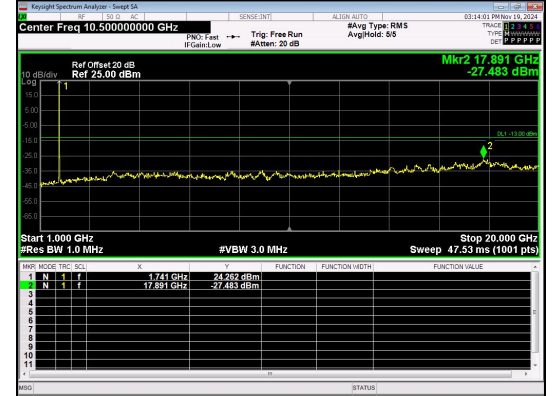
1000.0MHz-20000.0MHz Band 66 10MHz/1745.0/Mid 16QAM 1@0
