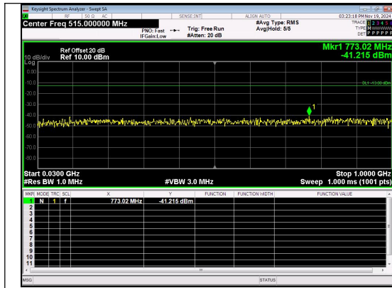
30.0MHz-1000.0MHz Band 66 15MHz/1772.5/High QPSK 1@0
