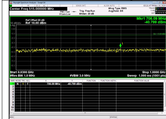
30.0MHz-1000.0MHz Band 66 10MHz/1715.0/Low QPSK 1@0
