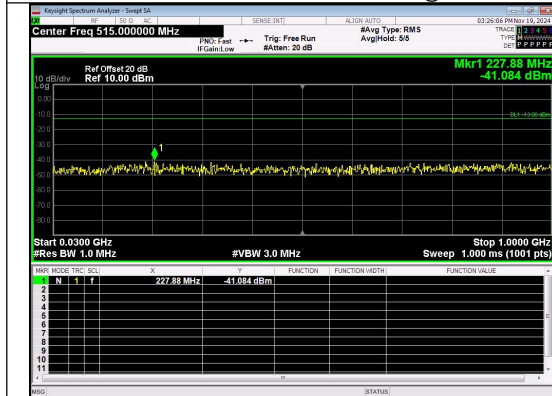
30.0MHz-1000.0MHz Band 66 15MHz/1745.0/Mid 16QAM 1@0
