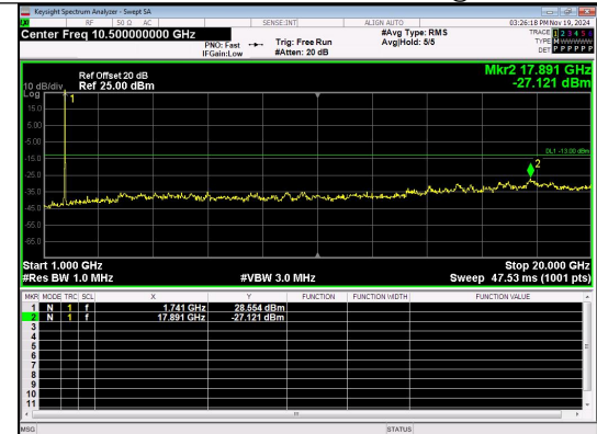
1000.0MHz-20000.0MHz Band 66 15MHz/1745.0/Mid 16QAM 1@0
