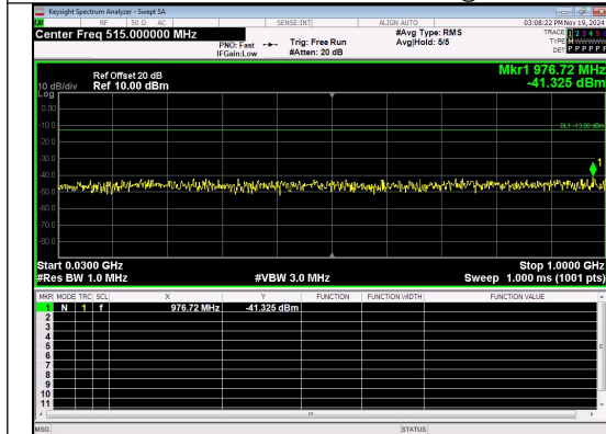
30.0MHz-1000.0MHz Band 66 5MHz/1745.0/Mid 16QAM 1@0
