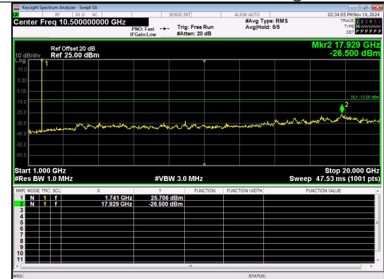
1000.0MHz-20000.0MHz Band 66 1.4MHz/1745.0/Mid 16QAM 1@0
