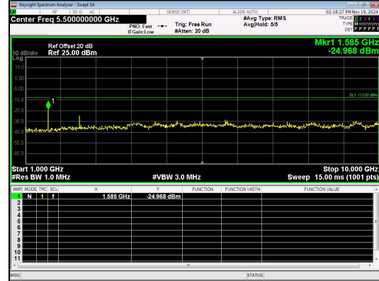
1000.0MHz-10000.0MHz Band 14 5MHz/795.5/High 16QAM 1@0
