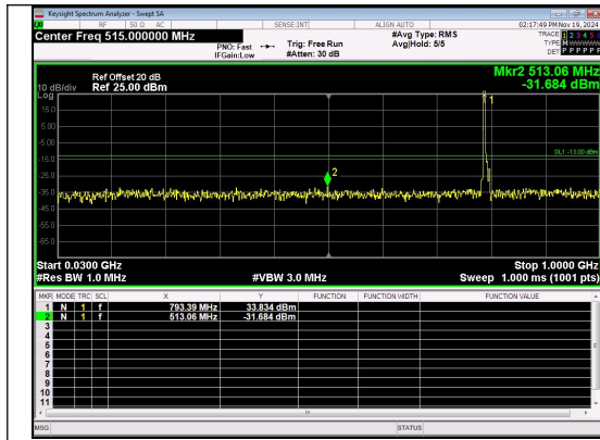
30.0MHz-1000.0MHz Band 14 5MHz/795.5/High QPSK 1@0
