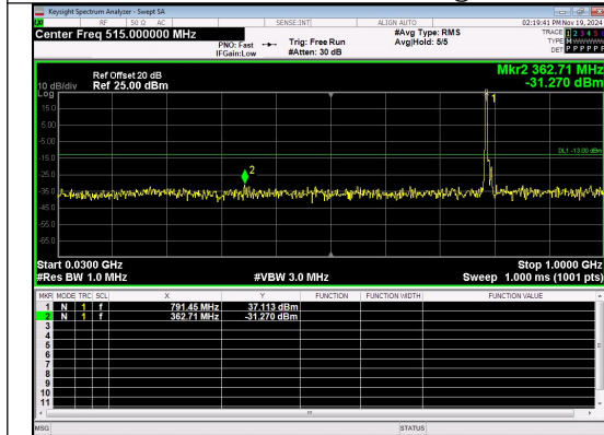
30.0MHz-1000.0MHz Band 14 5MHz/793.0/Mid 16QAM 1@0
