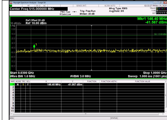
30.0MHz-1000.0MHz Band 66 1.4MHz/1745.0/Mid QPSK 1@0
