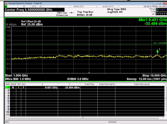
1000.0MHz-10000.0MHz Band 14 10MHz/793.0/Low 16QAM 1@0
