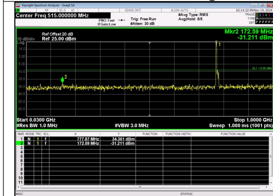
30.0MHz-1000.0MHz Band 13 10MHz/782.0/Low 16QAM 1@0
