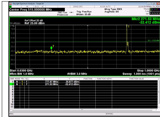
30.0MHz-1000.0MHz Band 13 10MHz/782.0/Mid QPSK 1@0
