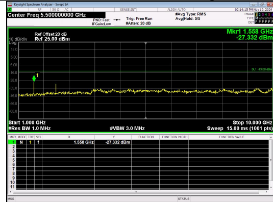
1000.0MHz-10000.0MHz Band 13 10MHz/782.0/Low QPSK 1@0
