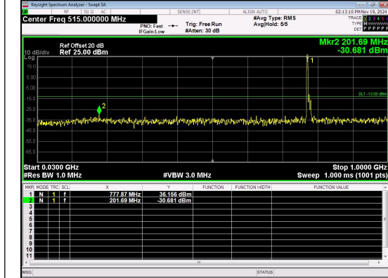
30.0MHz-1000.0MHz Band 13 10MHz/782.0/Mid 16QAM 1@0
