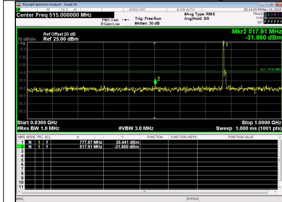
30.0MHz-1000.0MHz Band 13 10MHz/782.0/Low QPSK 1@0
