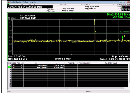
30.0MHz-1000.0MHz Band 12 10MHz/711.0/High QPSK 1@0
