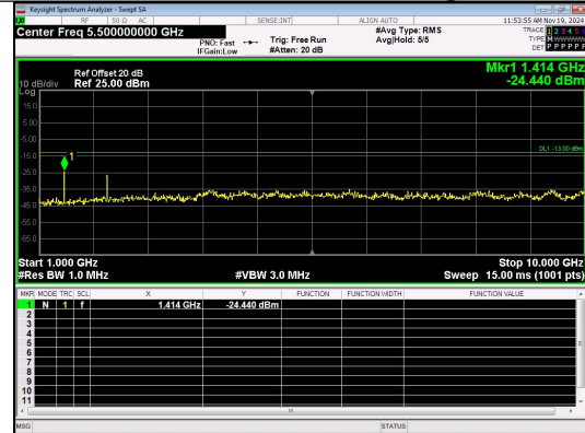
1000.0MHz-10000.0MHz Band 12 10MHz/711.0/High QPSK 1@0
