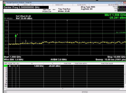
1000.0MHz-10000.0MHz Band 13 10MHz/782.0/Low 16QAM 1@0
