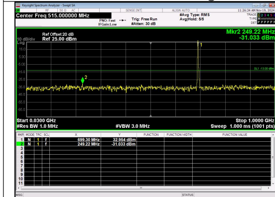
30.0MHz-1000.0MHz Band 12 3MHz/700.5/Low 16QAM 1@0
