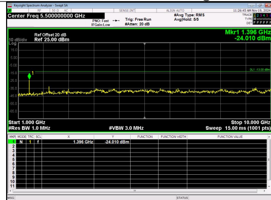
1000.0MHz-10000.0MHz Band 12 3MHz/700.5/Low 16QAM 1@0
