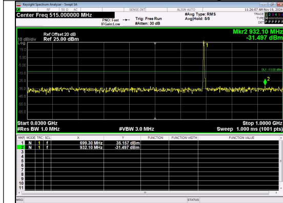
30.0MHz-1000.0MHz Band 12 3MHz/700.5/Low QPSK 1@0
