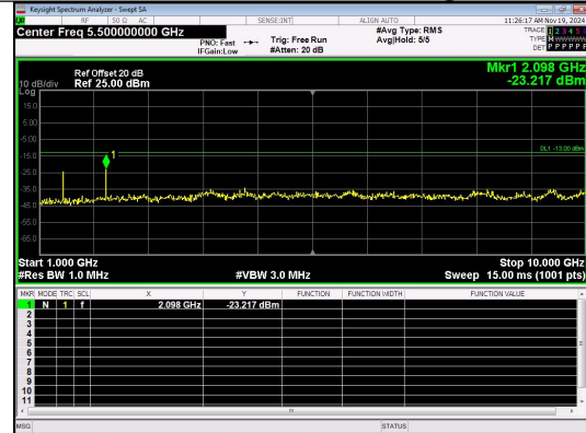
1000.0MHz-10000.0MHz Band 12 3MHz/700.5/Low QPSK 1@0
