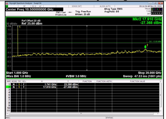
1000.0MHz-20000.0MHz Band 4 10MHz/1750.0/High 16QAM 1@0
