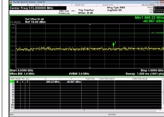
30.0MHz-1000.0MHz Band 4 10MHz/1732.5/Mid 16QAM 1@0
