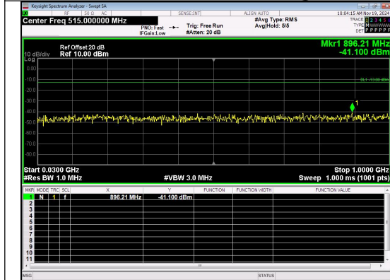
30.0MHz-1000.0MHz Band 4 20MHz/1720.0/Low QPSK 1@0
