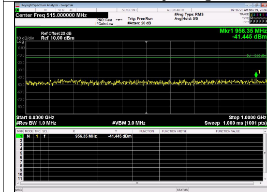
30.0MHz-1000.0MHz Band 4 10MHz/1750.0/High 16QAM 1@0
