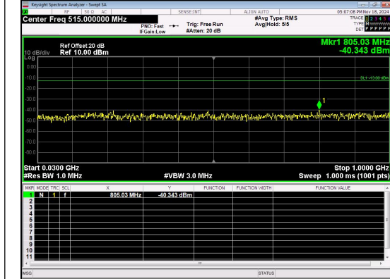
30.0MHz-1000.0MHz Band 4 5MHz/1712.5/Low 16QAM 1@0
