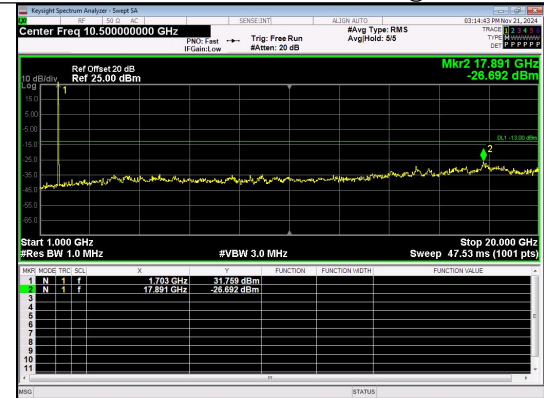
1000.0MHz-20000.0MHz Band 4 20MHz/1720.0/Low 16QAM 1@0
