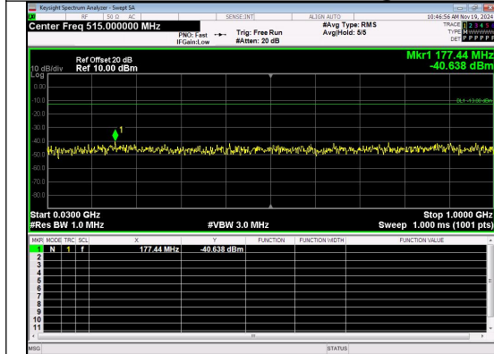
30.0MHz-1000.0MHz Band 4 10MHz/1715.0/Low QPSK 1@0
