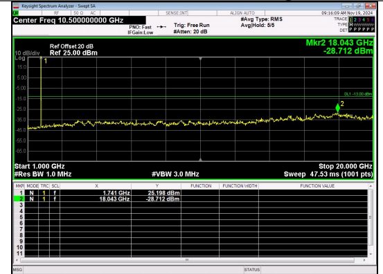
1000.0MHz-20000.0MHz Band 4 10MHz/1750.0/High QPSK 1@0
