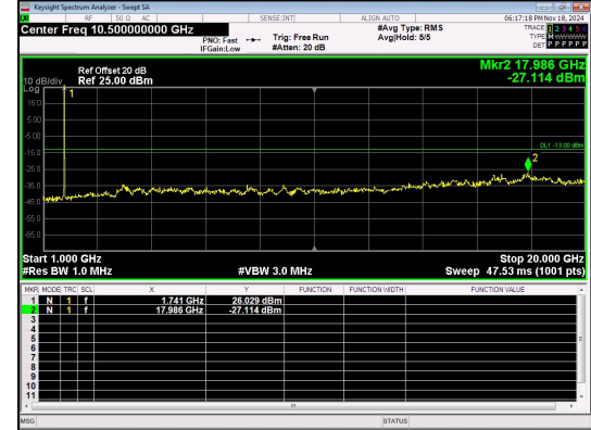
1000.0MHz-20000.0MHz Band 4 15MHz/1747.5/High 16QAM 1@0
