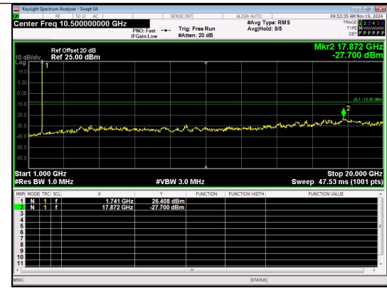
1000.0MHz-20000.0MHz Band 4 15MHz/1747.5/High QPSK 1@0
