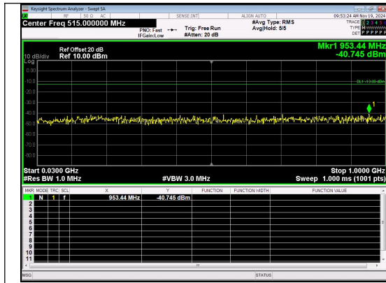
30.0MHz-1000.0MHz Band 4 15MHz/1747.5/High QPSK 1@0
