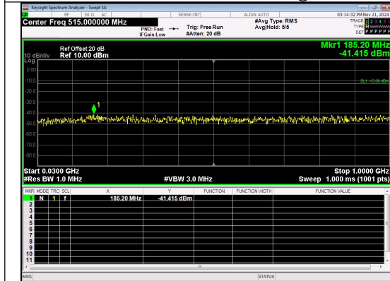
30.0MHz-1000.0MHz Band 4 20MHz/1720.0/Low 16QAM 1@0
