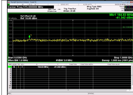
30.0MHz-1000.0MHz Band 4 15MHz/1732.5/Mid QPSK 1@0
