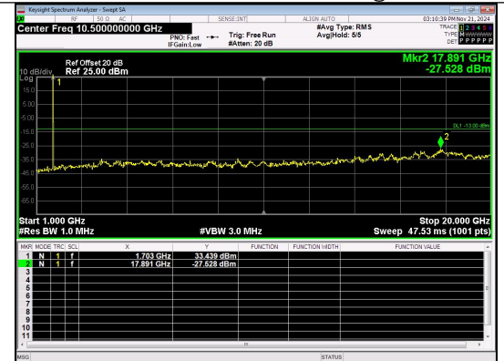
1000.0MHz-20000.0MHz Band 4 10MHz/1715.0/Low 16QAM 1@0
