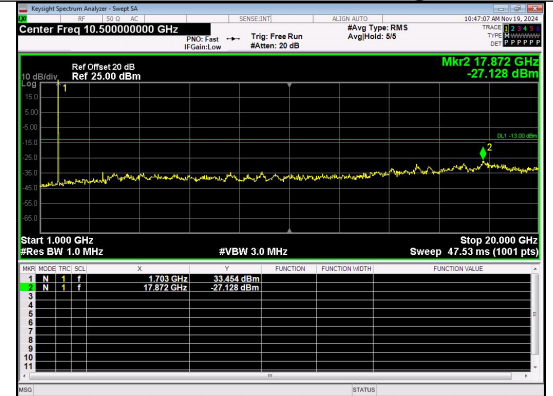
1000.0MHz-20000.0MHz Band 4 10MHz/1715.0/Low QPSK 1@0
