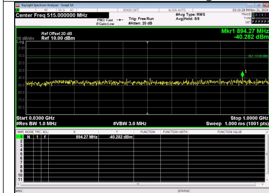
30.0MHz-1000.0MHz Band 4 10MHz/1715.0/Low 16QAM 1@0
