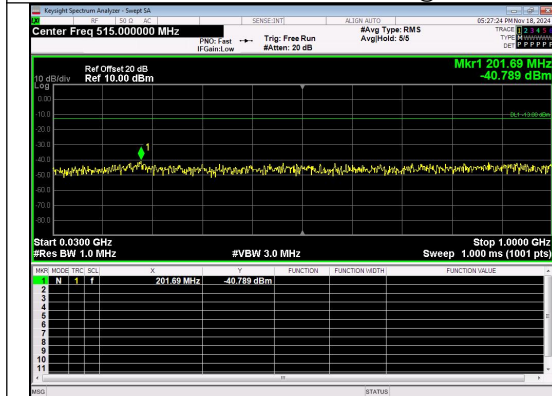
30.0MHz-1000.0MHz Band 4 15MHz/1732.5/Mid 16QAM 1@0
