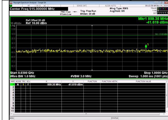
30.0MHz-1000.0MHz Band 4 10MHz/1750.0/High QPSK 1@0
