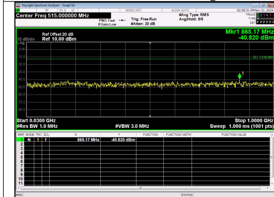
30.0MHz-1000.0MHz Band 2 20MHz/1860.0/Low QPSK 1@0
