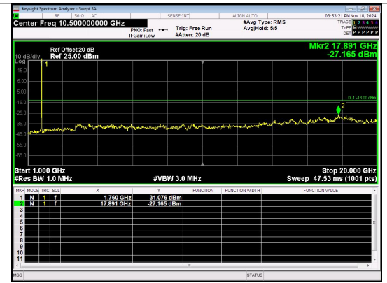
1000.0MHz-20000.0MHz Band 4 1.4MHz/1754.3/High QPSK 1@0
