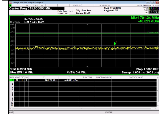
30.0MHz-1000.0MHz Band 4 3MHz/1753.5/High QPSK 1@0
