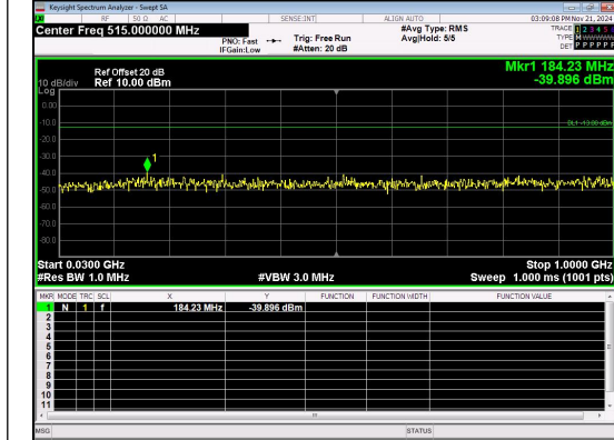
30.0MHz-1000.0MHz Band 4 1.4MHz/1710.7/Low 16QAM 1@0
