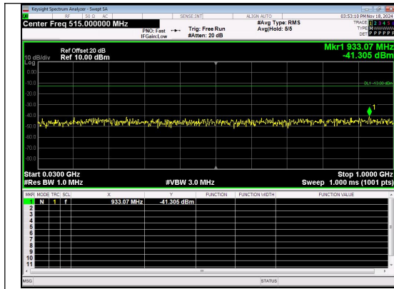
30.0MHz-1000.0MHz Band 4 1.4MHz/1754.3/High QPSK 1@0
