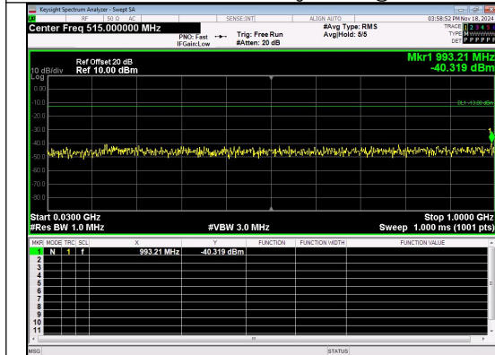
30.0MHz-1000.0MHz Band 4 3MHz/1753.5/High 16QAM 1@0
