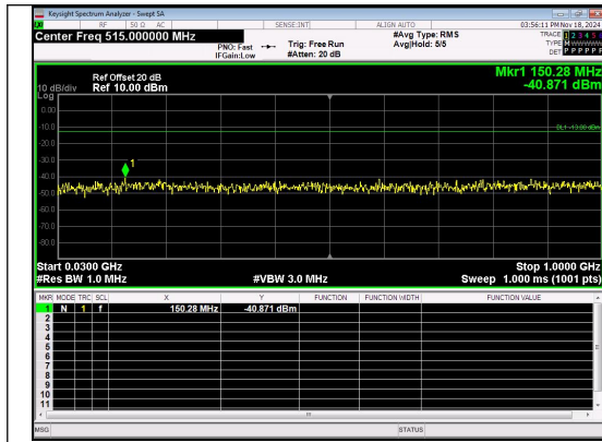
30.0MHz-1000.0MHz Band 4 1.4MHz/1710.7/Low QPSK 1@0
