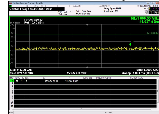
30.0MHz-1000.0MHz Band 4 1.4MHz/1732.5/Mid QPSK 1@0
