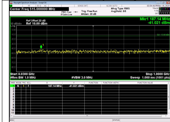
30.0MHz-1000.0MHz Band 4 1.4MHz/1754.3/High 16QAM 1@0
