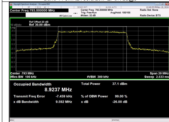
Band 14 10MHz/793.0/High QPSK 50@0
