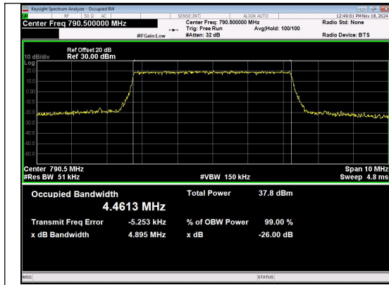
Band 14 5MHz/790.5/Low QPSK 25@0
