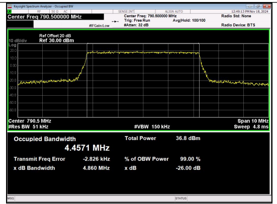
Band 14 5MHz/790.5/Low 16QAM 25@0
