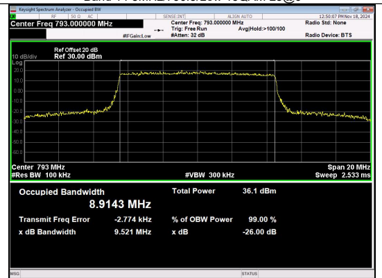
Band 14 10MHz/793.0/High 16QAM 50@0
