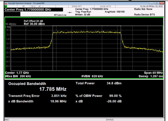
Band 66 20MHz/1770.0/High 16QAM 100@0
