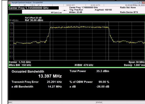
Band 66 15MHz/1745.0/Mid QPSK 75@0
