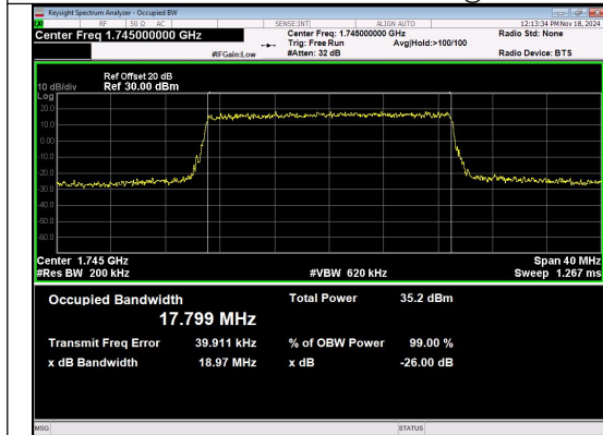
Band 4 20MHz/1745.0/High QPSK 100@0
