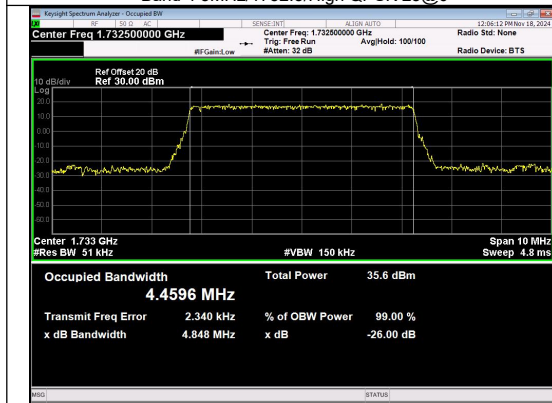
Band 4 5MHz/1732.5/Mid QPSK 25@0
