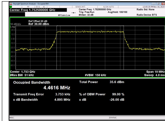
Band 4 5MHz/1752.5/High QPSK 25@0
