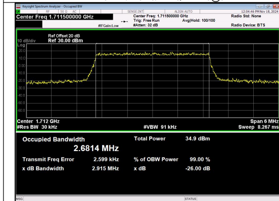
Band 4 3MHz/1711.5/Low QPSK 15@0
