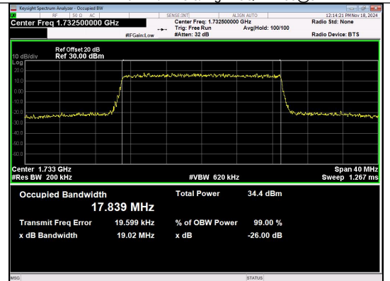
Band 4 20MHz/1732.5/Mid 16QAM 100@0
