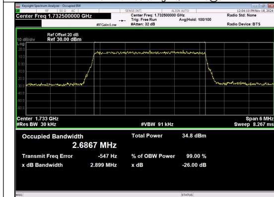
Band 4 3MHz/1732.5/Mid QPSK 15@0
