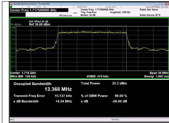
Band 4 15MHz/1717.5/Low QPSK 75@0
