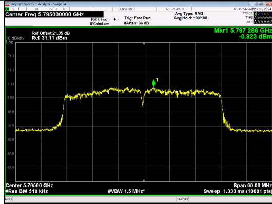
IEEE 802.11ac_Channel 159_40MHz_Antenna 4
