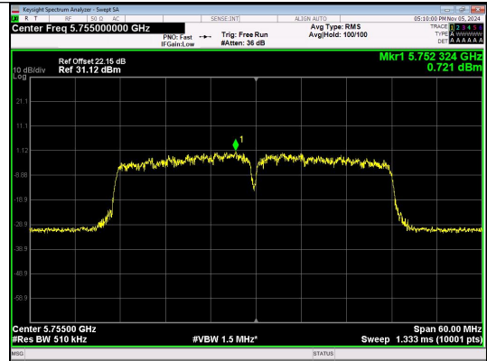
IEEE 802.11ac_Channel 151_40MHz_Antenna 4
