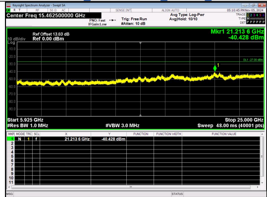
Spurious Emission:5925~25000.0 MHz IEEE 802.11ac Channel 151 40MHz Antenna 4
