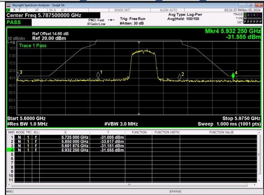
Out Of Band Emission IEEE 802.11n Channel 159 40MHz Antenna 4
