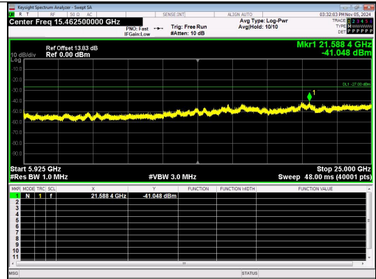
Spurious Emission:5925~25000.0 MHz IEEE 802.11n_Channel 159_40MHz_Antenna 4
