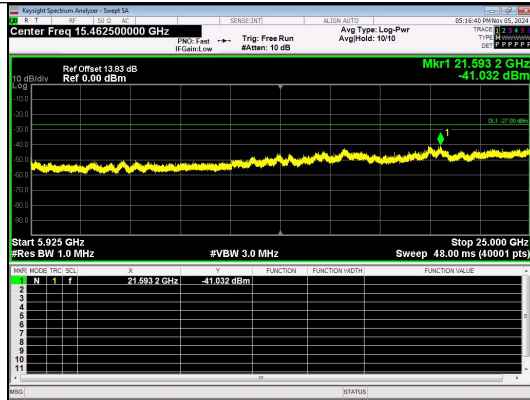
Spurious Emission:5925~25000.0 MHz IEEE 802.11ac Channel 159 40MHz Antenna 4
