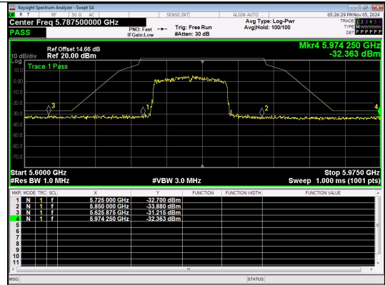
Out Of Band Emission IEEE 802.11ac Channel 155 80MHz Antenna 4
