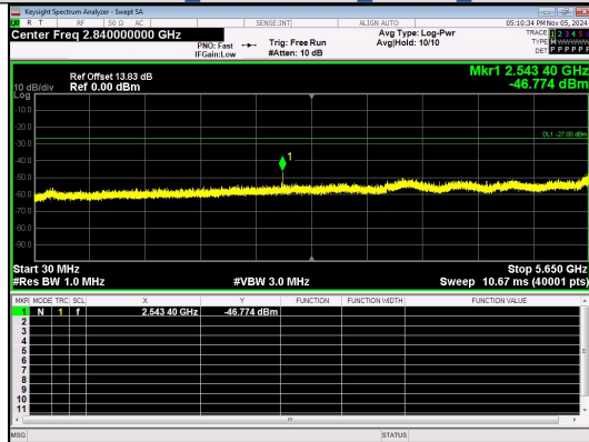
Spurious Emission:30.0~5650 MHz IEEE 802.11ac Channel 151 40MHz Antenna 4
