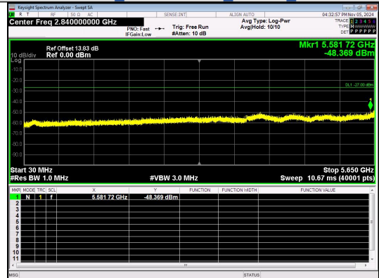
Spurious Emission:30.0~5650 MHz IEEE 802.11ac_Channel 149_20MHz_Antenna 4
