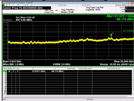
Spurious Emission:5925~25000.0 MHz IEEE 802.11ac Channel 165 20MHz Antenna 4
