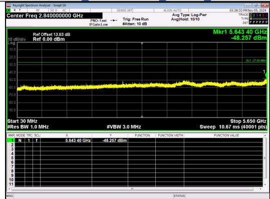
Spurious Emission: 30.0~5650 MHz IEEE 802.11n Channel 151 40MHz Antenna 4
