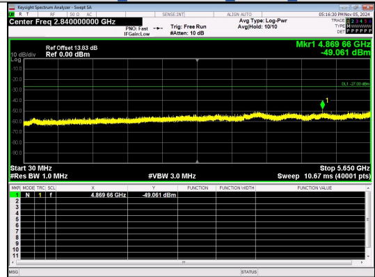
Spurious Emission:30.0~5650 MHz IEEE 802.11ac Channel 159 40MHz Antenna 4
