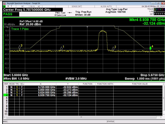
Out Of Band Emission IEEE 802.11ac Channel 165 20MHz Antenna 4
