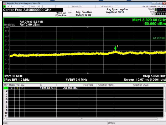
Spurious Emission: 30.0~5650 MHz IEEE 802.11n Channel 165 20MHz Antenna 4
