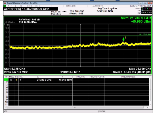
Spurious Emission: 5925~25000.0 MHz IEEE 802.11n Channel 165 20MHz Antenna 4
