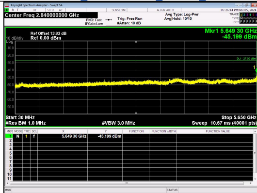
Spurious Emission:30.0~5650 MHz IEEE 802.11ac Channel 155 80MHz Antenna 4
