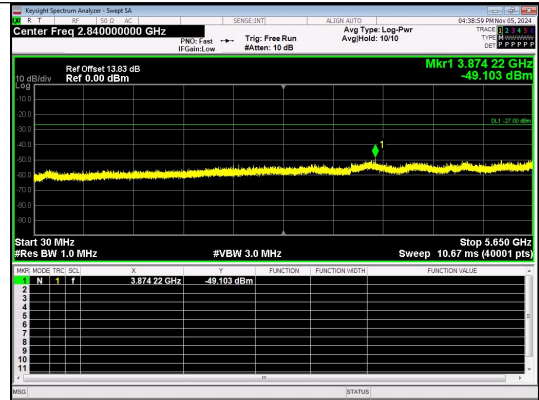
Spurious Emission:30.0~5650 MHz IEEE 802.11ac Channel 165 20MHz Antenna 4
