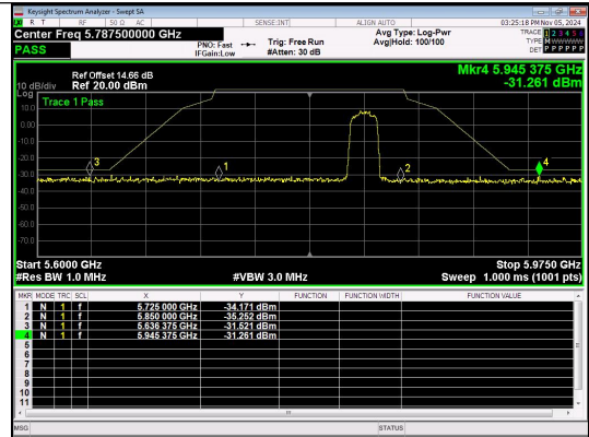
Out Of Band Emission IEEE 802.11n Channel 165 20MHz Antenna 4
