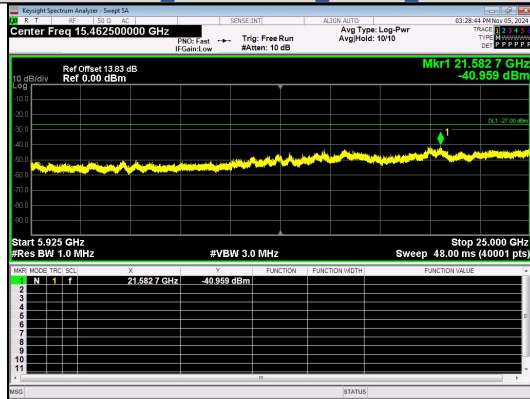
Spurious Emission: 5925~25000.0 MHz IEEE 802.11n Channel 151 40MHz Antenna 4
