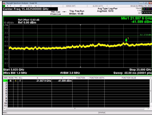
Spurious Emission: 5925~25000.0 MHz IEEE 802.11n Channel 157 20MHz Antenna 4
