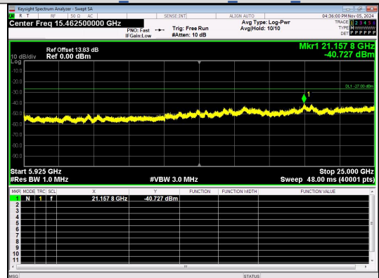
Spurious Emission:5925~25000.0 MHz IEEE 802.11ac Channel 157 20MHz Antenna 4
