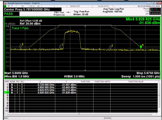
Out Of Band Emission IEEE 802.11ac Channel 151 40MHz Antenna 4
