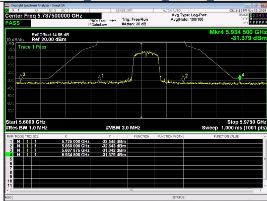
Out Of Band Emission IEEE 802.11ac Channel 159 40MHz Antenna 4
