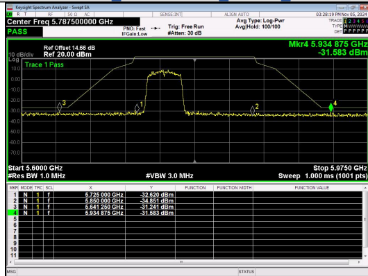
Out Of Band Emission IEEE 802.11n Channel 151 40MHz Antenna 4
