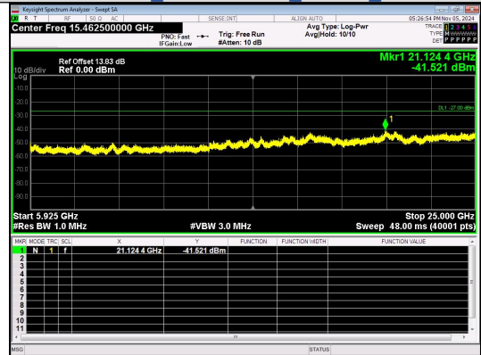
Spurious Emission:5925~25000.0 MHz IEEE 802.11ac Channel 155 80MHz Antenna 4
