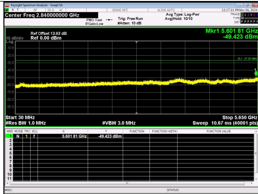
Spurious Emission:30.0~5650 MHz IEEE 802.11ac Channel 157 20MHz Antenna 3
