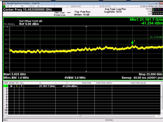
Spurious Emission:5925~25000.0 MHz IEEE 802.11ac Channel 165 20MHz Antenna 3
