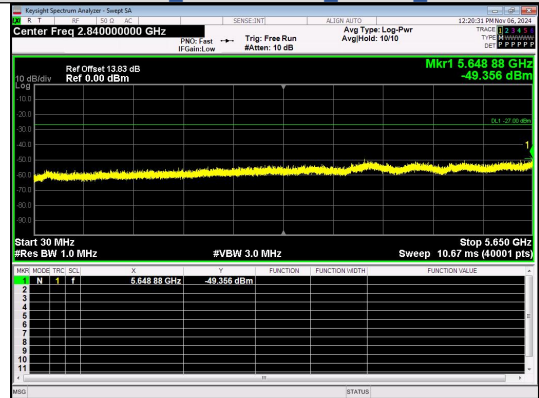
Spurious Emission:30.0~5650 MHz IEEE 802.11ac Channel 165 20MHz Antenna 3
