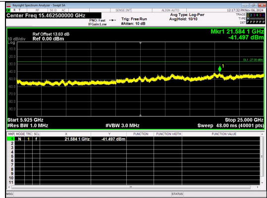
Spurious Emission:5925~25000.0 MHz IEEE 802.11ac Channel 157 20MHz Antenna 3
