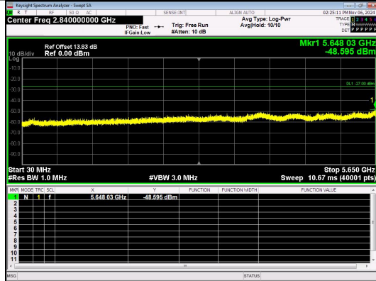
Spurious Emission:30.0~5650 MHz IEEE 802.11ac Channel 151 40MHz Antenna 3
