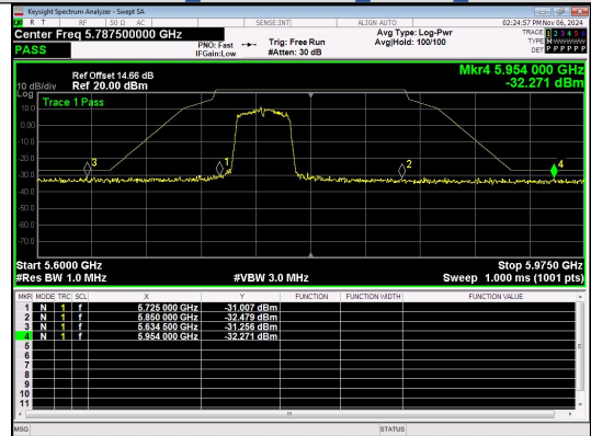
Out Of Band Emission IEEE 802.11ac Channel 151 40MHz Antenna 3
