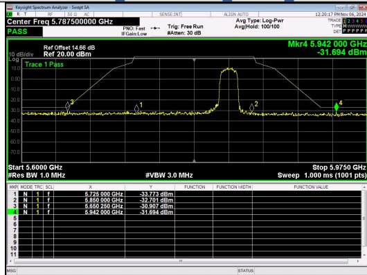
Out Of Band Emission IEEE 802.11ac Channel 165 20MHz Antenna 3
