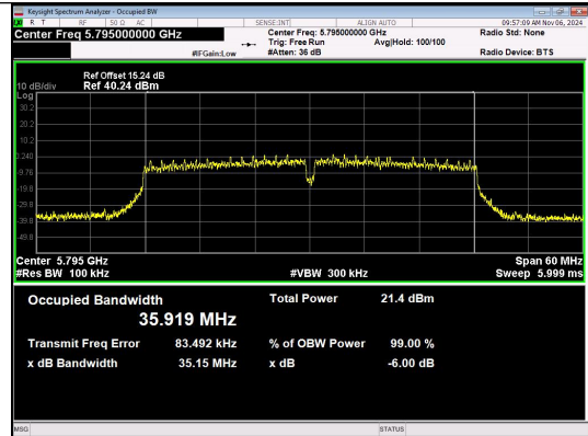
IEEE 802.11n Channel 159 40MHz Antenna 3
