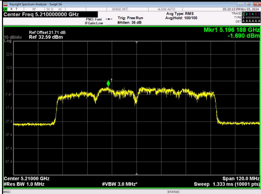
IEEE 802.11ac_Channel 42_80MHz_Antenna 4
