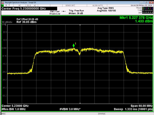
IEEE 802.11ac_Channel 46_40MHz_Antenna 4
