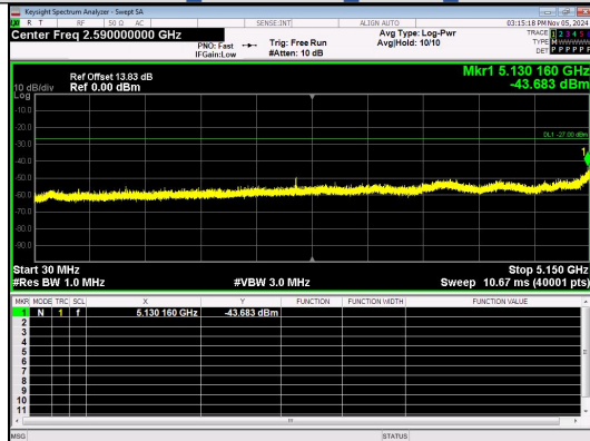
Spurious Emission:30.0~5150 MHz IEEE 802.11n Channel 48 20MHz Antenna 4
