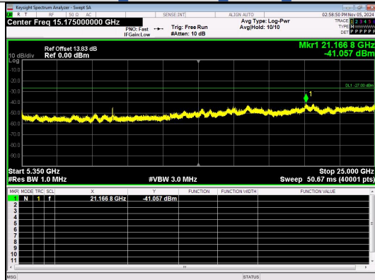
Spurious Emission:5350~25000.0 MHz IEEE 802.11n Channel 40 20MHz Antenna 4
