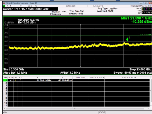
Spurious Emission:5350~25000.0 MHz IEEE 802.11ac Channel 48 20MHz Antenna 4
