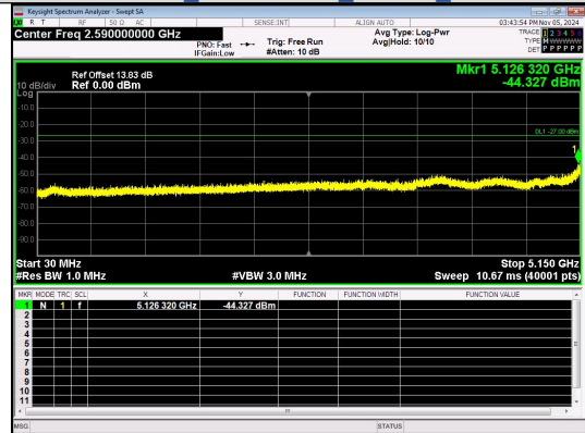
Spurious Emission:30.0~5150 MHz IEEE 802.11a Channel 48 20MHz Antenna 4
