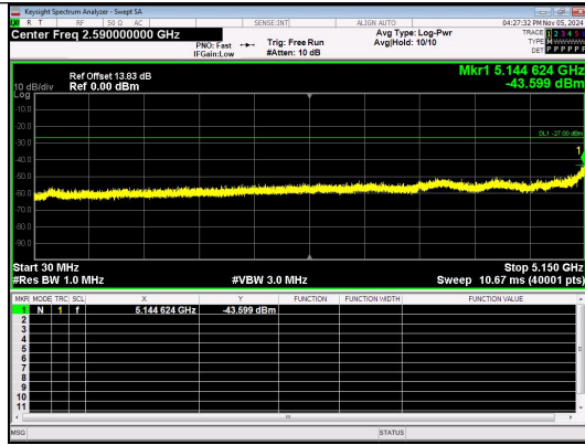
Spurious Emission:30.0~5150 MHz IEEE 802.11ac Channel 40 20MHz Antenna 4
