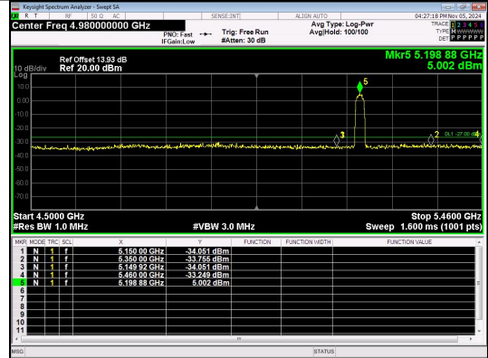
Out Of Band Emission IEEE 802.11ac Channel 40 20MHz Antenna 4
