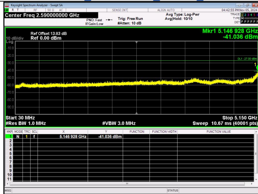
Spurious Emission:30.0~5150 MHz IEEE 802.11ac Channel 38 40MHz Antenna 4
