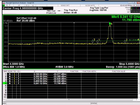
Out Of Band Emission IEEE 802.11a Channel 48 20MHz Antenna 4
