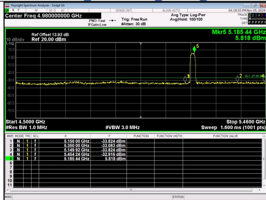
Out Of Band Emission IEEE 802.11ac Channel 36 20MHz Antenna 4
