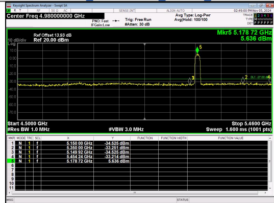
Out Of Band Emission IEEE 802.11n Channel 36 20MHz Antenna 4
