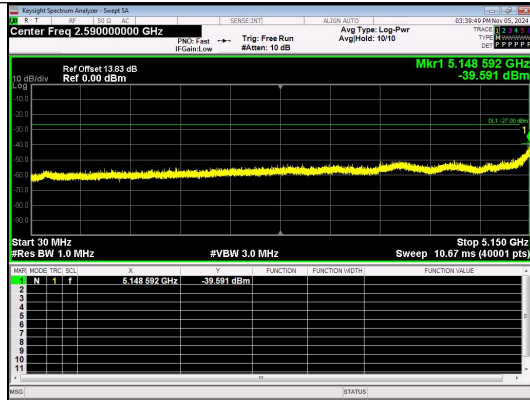
Spurious Emission:30.0~5150 MHz IEEE 802.11a Channel 40 20MHz Antenna 4
