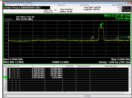
Out Of Band Emission IEEE 802.11n Channel 46 40MHz Antenna 4
