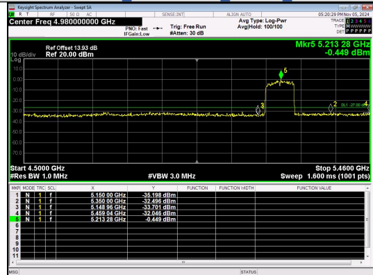
Out Of Band Emission IEEE 802.11ac Channel 42 80MHz Antenna 4
