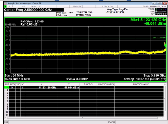
Spurious Emission:30.0~5150 MHz IEEE 802.11ac Channel 48 20MHz Antenna 4
