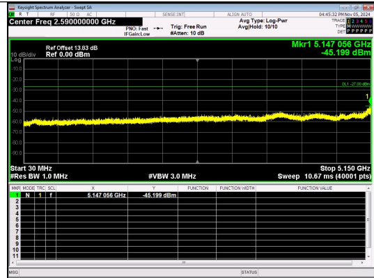
Spurious Emission:30.0~5150 MHz IEEE 802.11ac Channel 46 40MHz Antenna 4
