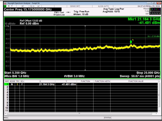
Spurious Emission:5350~25000.0 MHz IEEE 802.11ac Channel 40 20MHz Antenna 4
