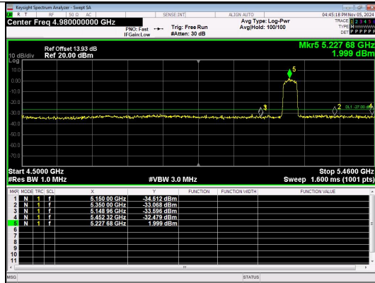
Out Of Band Emission IEEE 802.11ac Channel 46 40MHz Antenna 4
