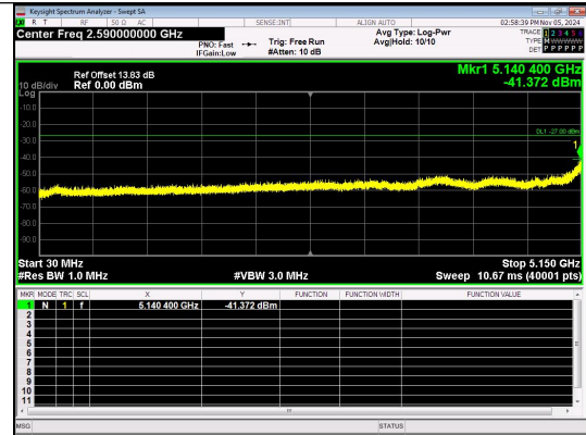
Spurious Emission:30.0~5150 MHz IEEE 802.11n Channel 40 20MHz Antenna 4
