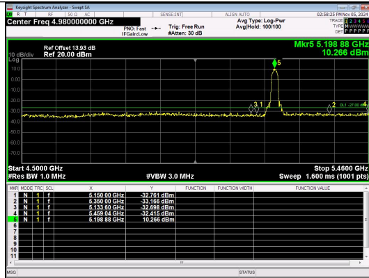
Out Of Band Emission IEEE 802.11n Channel 40 20MHz Antenna 4
