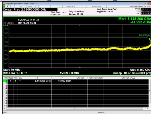
Spurious Emission:30.0~5150 MHz IEEE 802.11n Channel 36 20MHz Antenna 4
