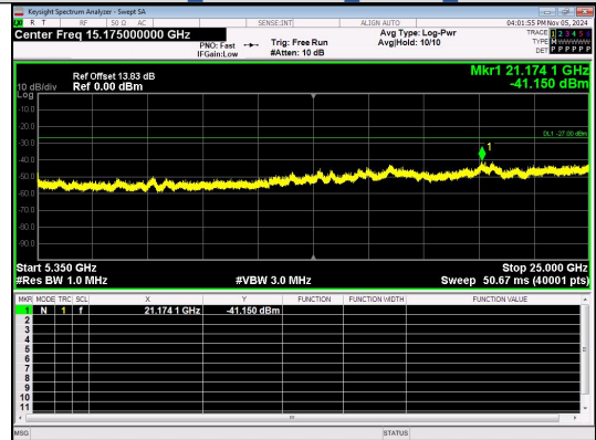
Spurious Emission: 5350~25000.0 MHz IEEE 802.11n Channel 46 40MHz Antenna 4
