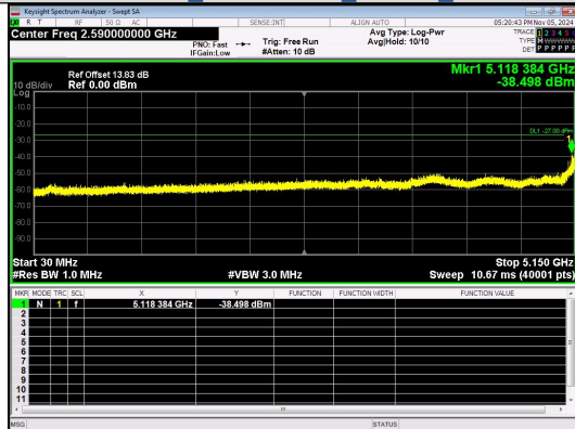
Spurious Emission:30.0~5150 MHz IEEE 802.11ac Channel 42 80MHz Antenna 4
