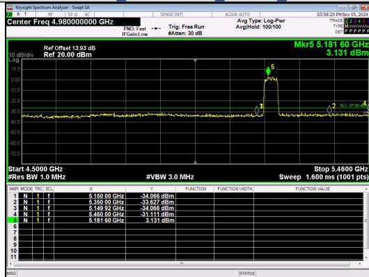
Out Of Band Emission IEEE 802.11n Channel 38 40MHz Antenna 4
