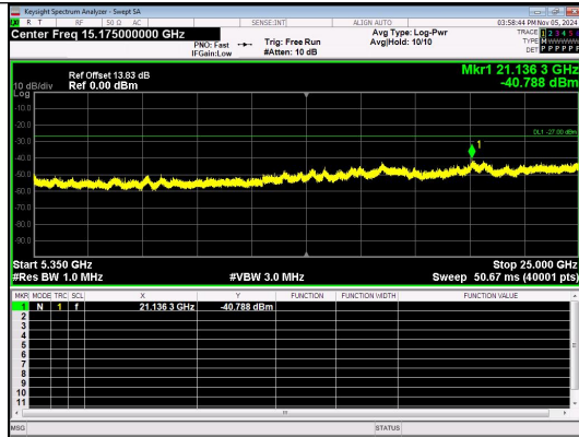
Spurious Emission: 5350~25000.0 MHz IEEE 802.11n Channel 38 40MHz Antenna 4
