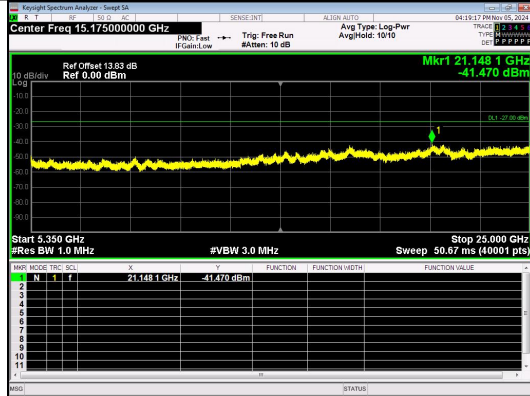
Spurious Emission: 5350~25000.0 MHz IEEE 802.11ac Channel 36 20MHz Antenna 4
