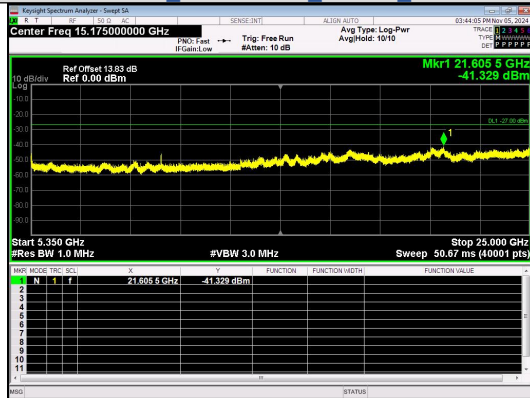
Spurious Emission:5350~25000.0 MHz IEEE 802.11a Channel 48 20MHz Antenna 4
