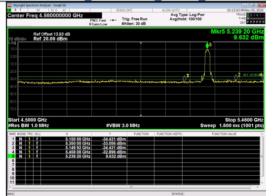
Out Of Band Emission IEEE 802.11n Channel 48 20MHz Antenna 4
