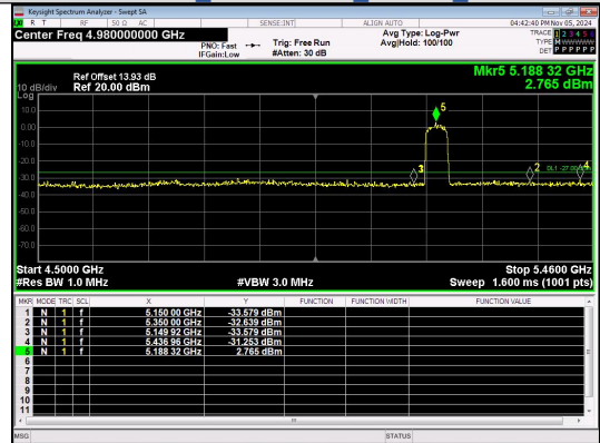
Out Of Band Emission IEEE 802.11ac Channel 38 40MHz Antenna 4
