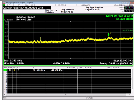
Spurious Emission:5350~25000.0 MHz IEEE 802.11a Channel 40 20MHz Antenna 4
