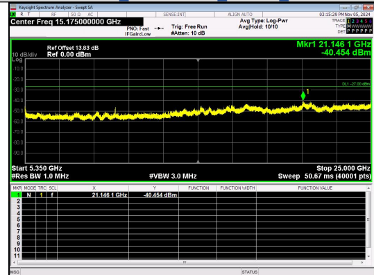
Spurious Emission:5350~25000.0 MHz IEEE 802.11n Channel 48 20MHz Antenna 4
