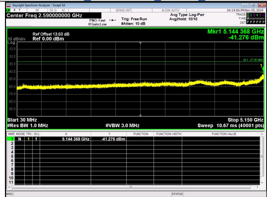
Spurious Emission: 30.0~5150 MHz IEEE 802.11ac Channel 36 20MHz Antenna 4
