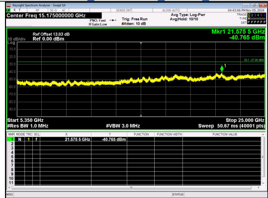
Spurious Emission:5350~25000.0 MHz IEEE 802.11ac Channel 38 40MHz Antenna 4
