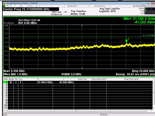
Spurious Emission:5350~25000.0 MHz IEEE 802.11ac Channel 46 40MHz Antenna 4
