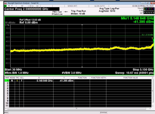
Spurious Emission:30.0~5150 MHz IEEE 802.11n Channel 38 40MHz Antenna 4
