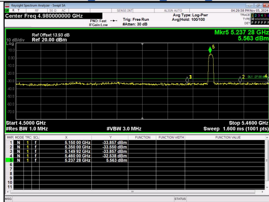
Out Of Band Emission IEEE 802.11ac Channel 48 20MHz Antenna 4
