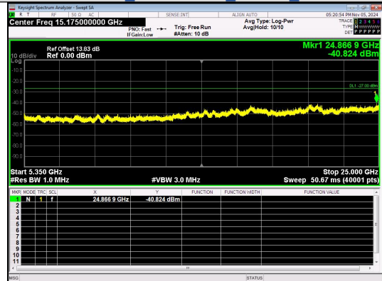
Spurious Emission:5350~25000.0 MHz IEEE 802.11ac Channel 42 80MHz Antenna 4
