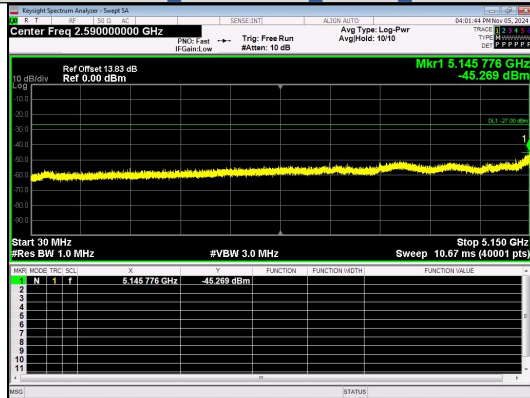
Spurious Emission: 30.0~5150 MHz IEEE 802.11n Channel 46 40MHz Antenna 4
