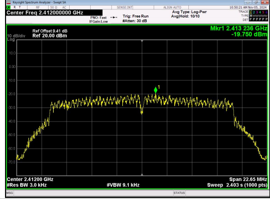
IEEE 802.11g_Channel 1_20MHz_Antenna 2
