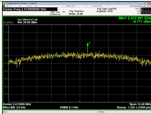
IEEE 802.11b_Channel 1_20MHz_Antenna 2
