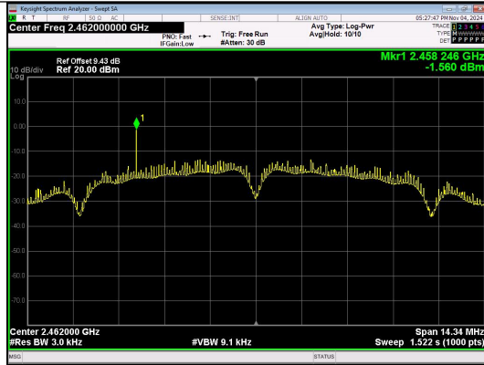
IEEE 802.11b Channel 11 20MHz Antenna 1
