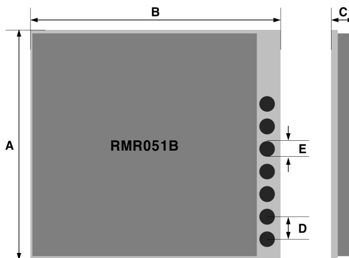
Figure 2. Mechanical Outline
