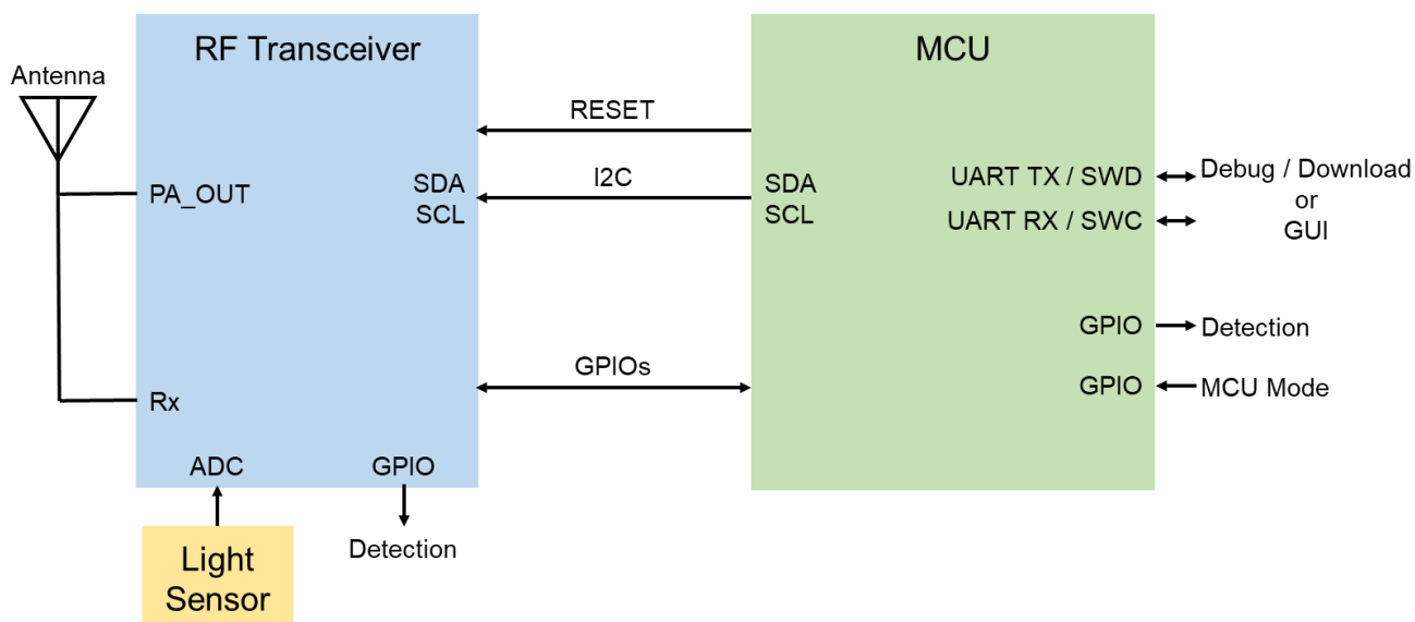
Figure 3. Block Diagram
