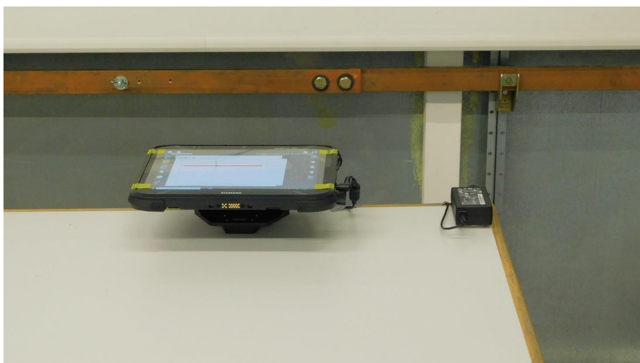
Picture 10: Test setup AC power line conducted emissions (front view)
