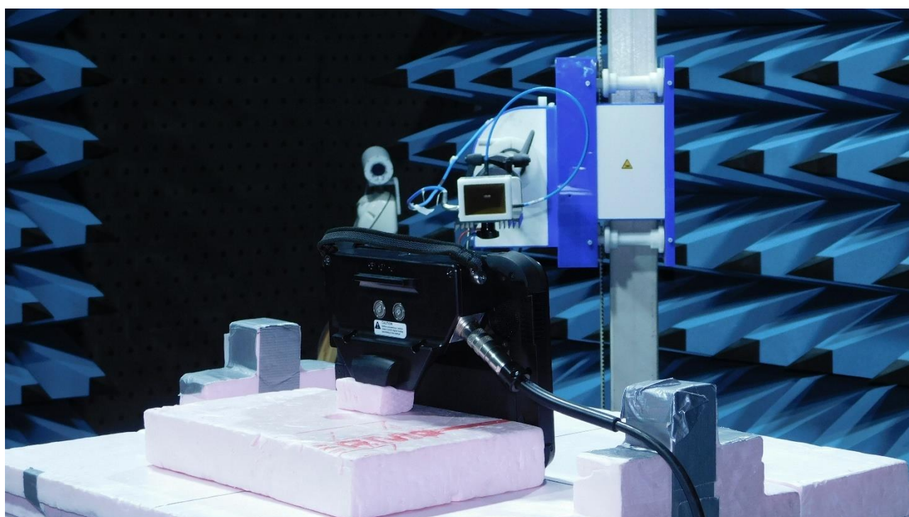
Picture 8: FS-SAC, radiated emission test 17 GHz – 26 GHz (rear view)
