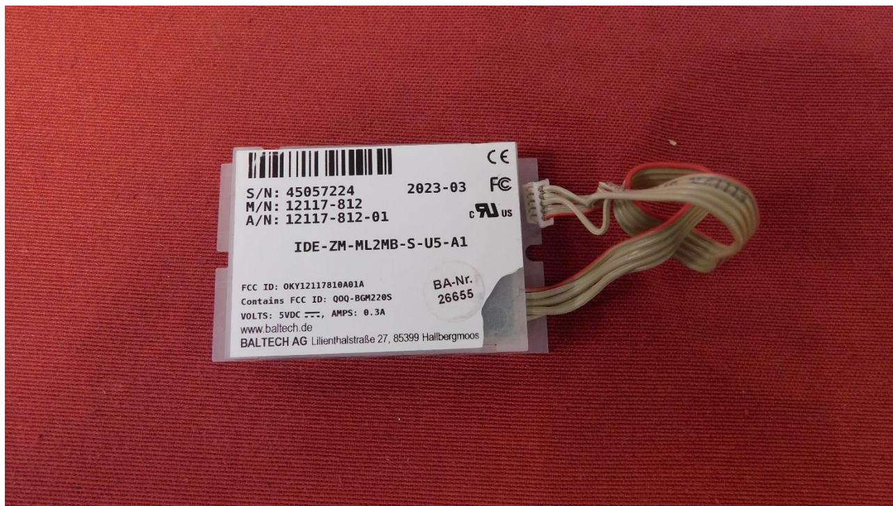
Picture 3: RFID module in cabinet top side
