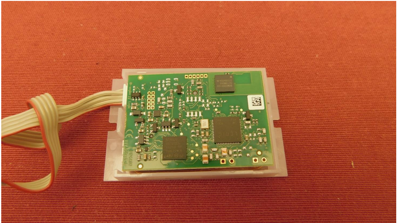
Picture 5: PCB of RFID module top side
