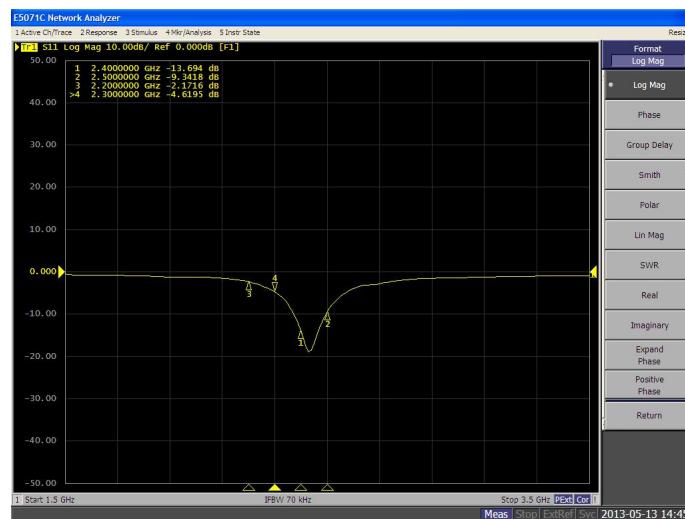
图 3 Mouse Antenna S11
