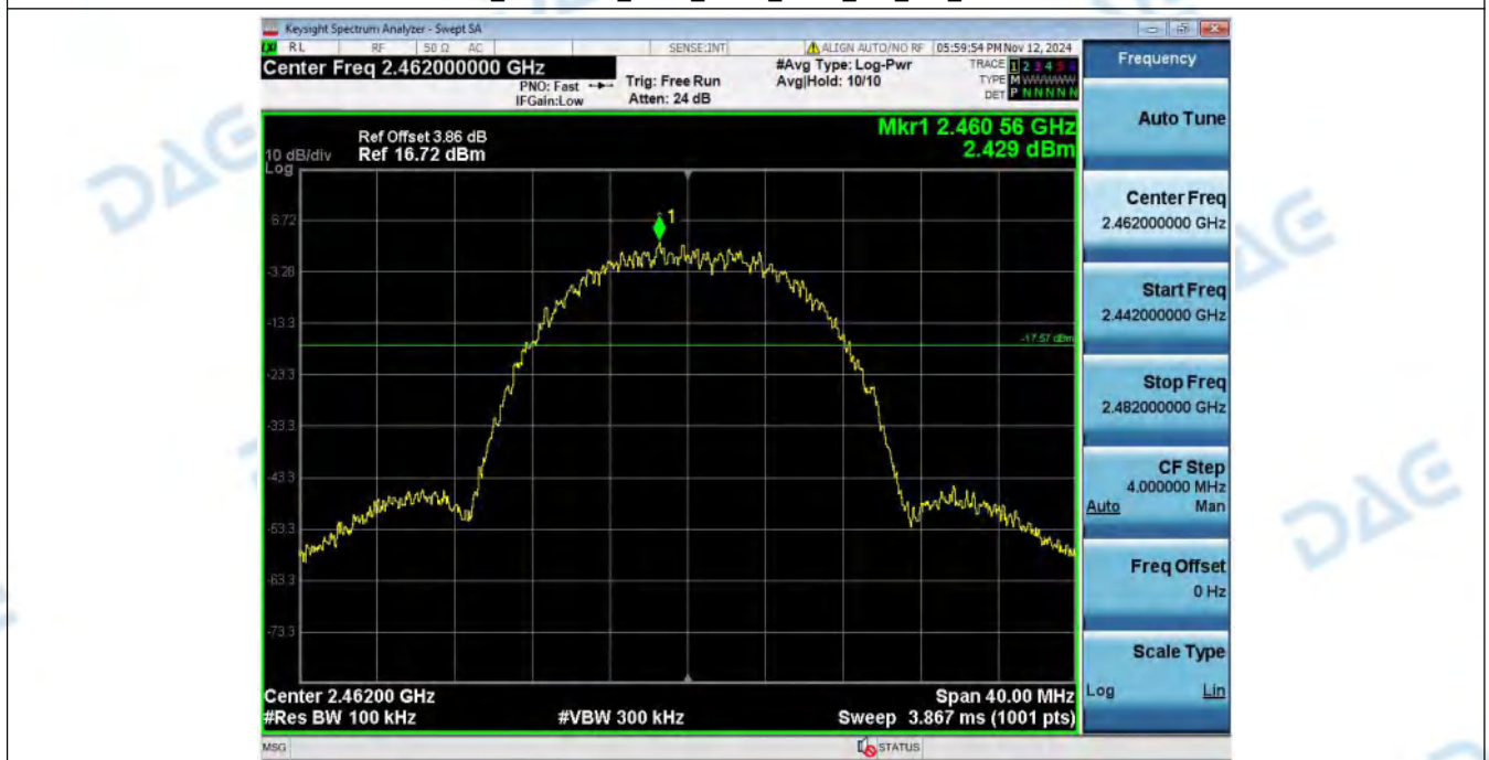
2_Spurious_Emission_NVNT_ANT1_802_11b_2462
