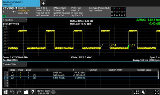
IEEE 802.11n 40MHz Channel 6
