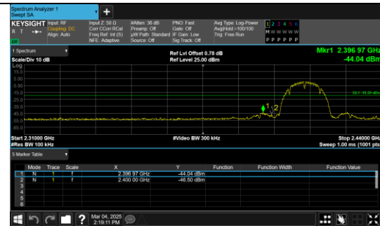
Out Of Band Emission IEEE 802.11b Channel 1 20MHz Antenna 0
