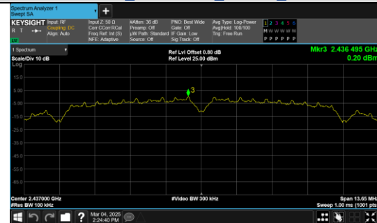
In-Band Reference Level IEEE 802.11b Channel 6 20MHz Antenna 0
