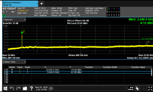
30.0 MHz - 25000.0 MHz IEEE 802.11n Channel 6_40MHz_Antenna 0
