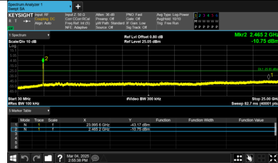
30.0 MHz - 25000.0 MHz IEEE 802.11n Channel 9_40MHz_Antenna 0
