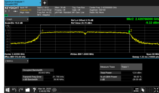
IEEE 802.11n Channel 3 40MHz Antenna 0
