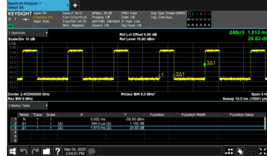
IEEE 802.11n 40MHz Channel 9
