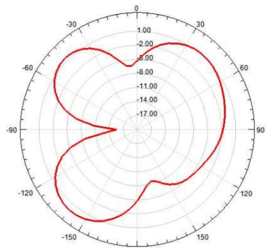
Radiation Pattern 2
