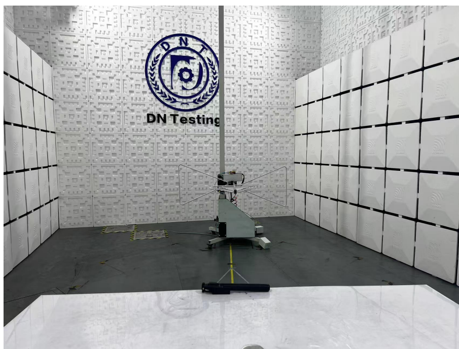
Radiated Emission Test View|(Below 1G)
