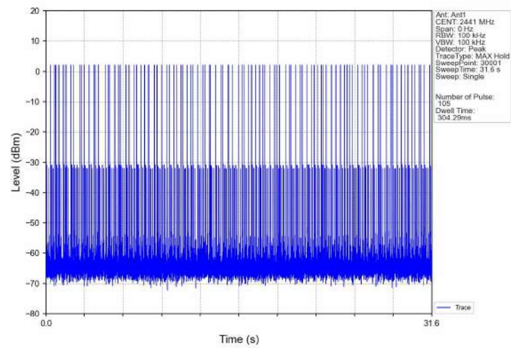
Dwell_Time_(Hopping)_NVNT_ANT1_DH5_2441_Accumulated
