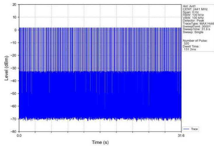
Dwell_Time_(Hopping)_NVNT_ANT1_2-DH1_2441_Accumulated
