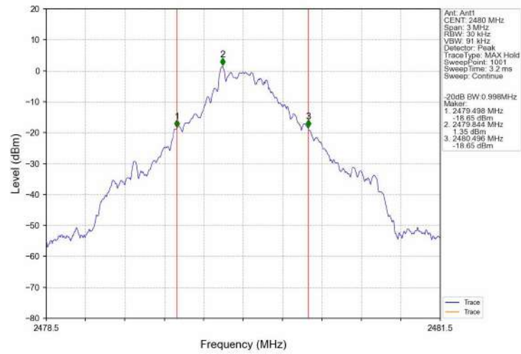
-20dB_Bandwidth_NVNT_ANT1_DH5_2480
