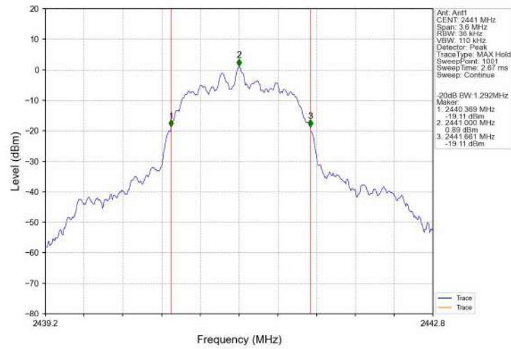
-20dB_Bandwidth_NVNT_ANT1_2-DH5_2441
