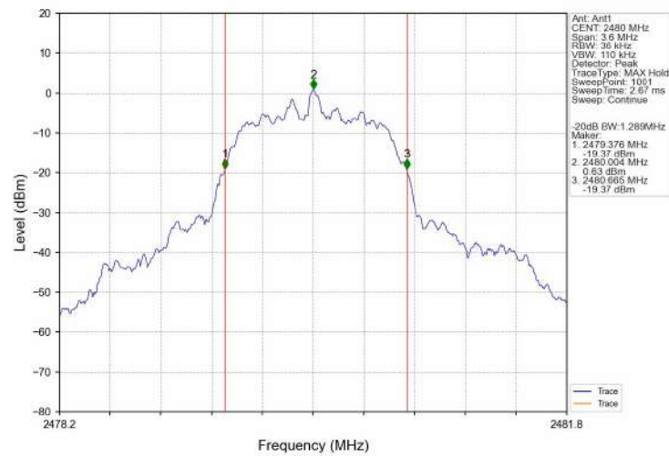
-20dB_Bandwidth_NVNT_ANT1_2-DH5_2480
