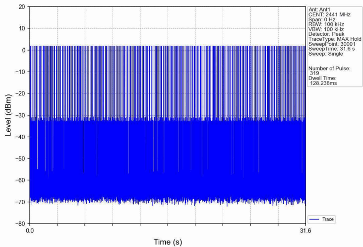
Dwell_Time_(Hopping)_NVNT_ANT1_1-DH1_2441_Accumulated
