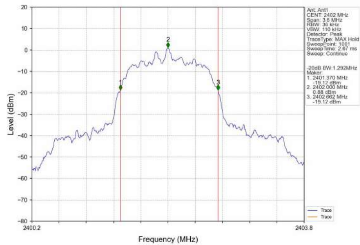
-20dB_Bandwidth_NVNT_ANT1_2-DH5_2402
