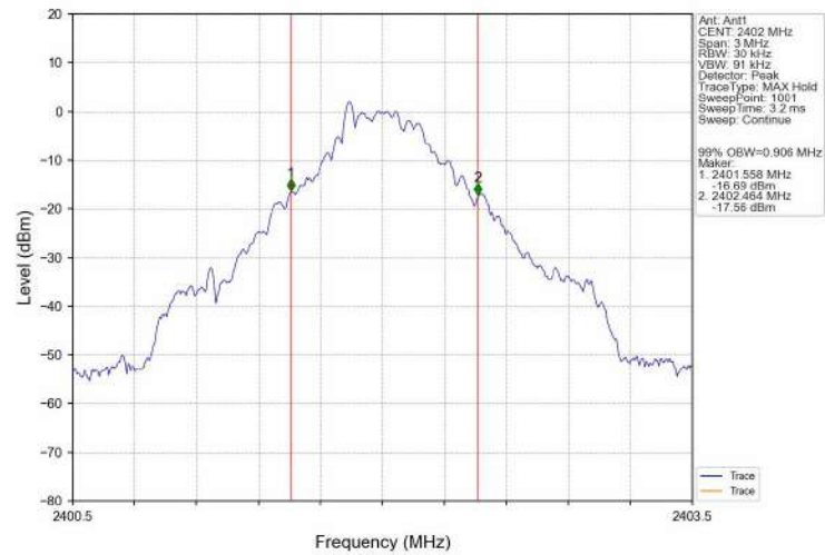
99%_Occupied_Bandwidth_NVNT_ANT1_DH5_2402
