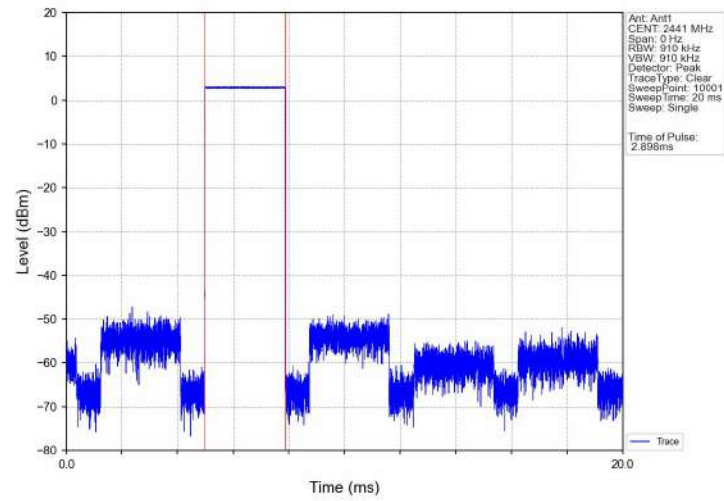
Dwell_Time_(Hopping)_NVNT_ANT1_DH5_2441_Accumulated
