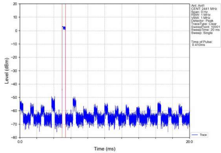
Dwell_Time_(Hopping)_NVNT_ANT1_2-DH1_2441_Accumulated
