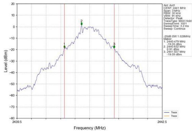
-20dB_Bandwidth_NVNT_ANT1_DH5_2441
