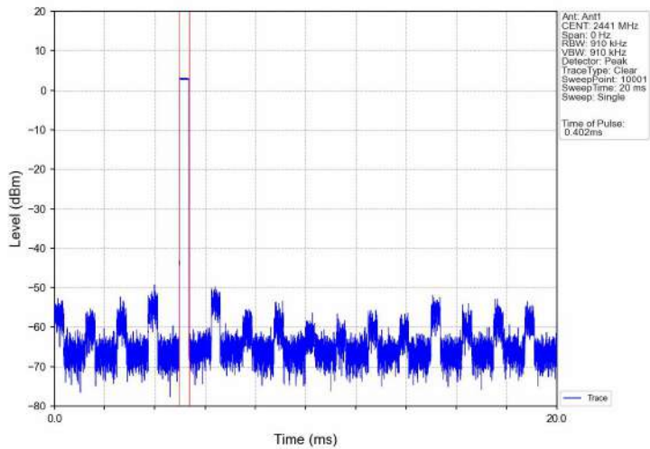
Dwell_Time_(Hopping)_NVNT_ANT1_1-DH1_2441_Accumulated
