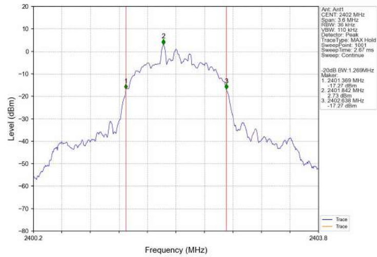
-20dB_Bandwidth_NVNT_ANT1_3-DH5_2402
