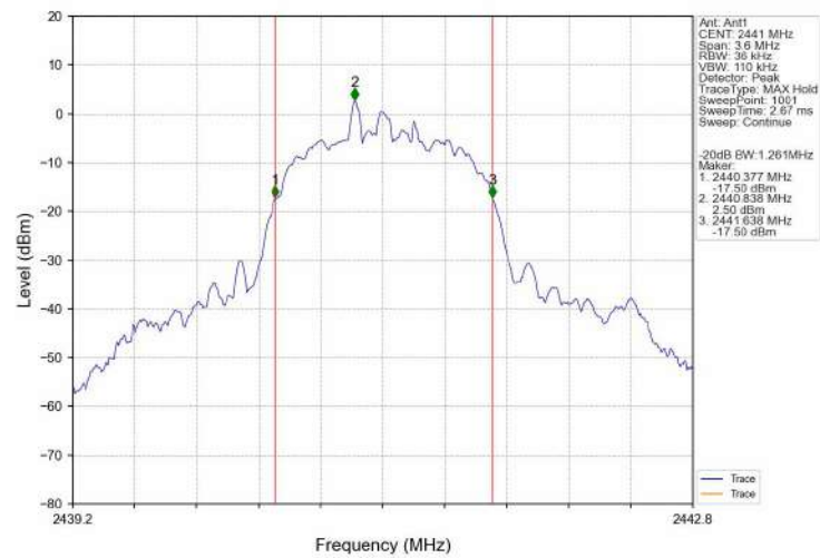
-20dB_Bandwidth_NVNT_ANT1_3-DH5_2441
