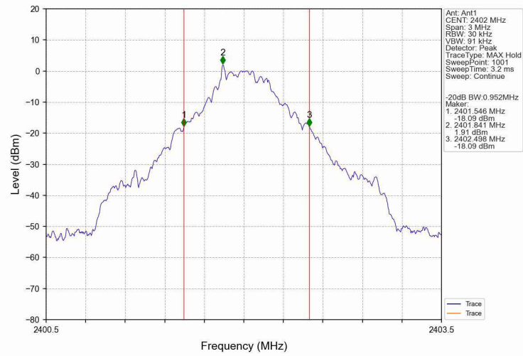
-20dB_Bandwidth_NVNT_ANT1_DH5_2402
