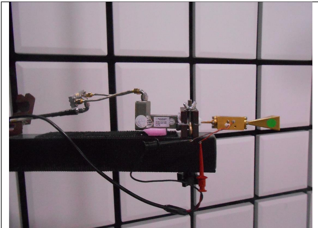
RF Radiated_ 75 – 100 GHz
