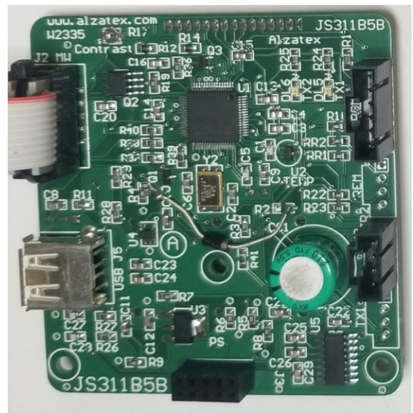
Main Microprocessor and Control PCB
