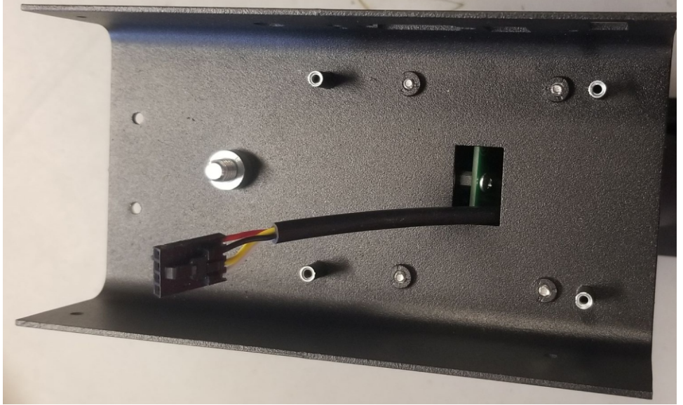
Trigger switch and Battery Holder
