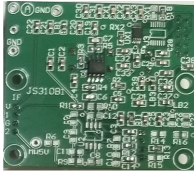
Microwave Input Amplifier and A2D PCB
