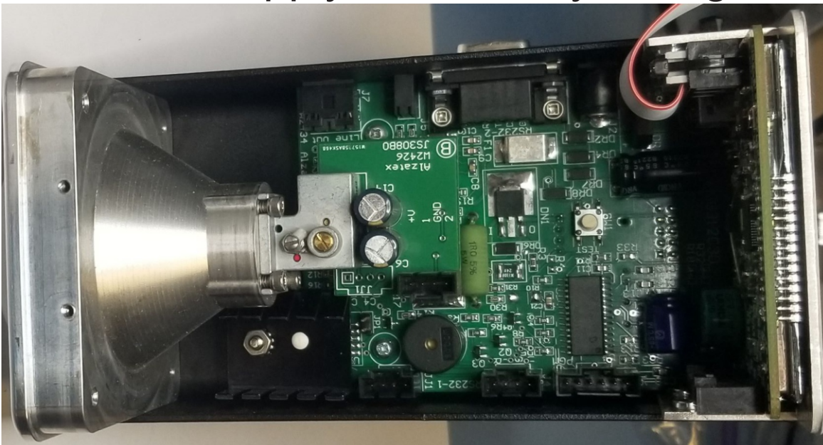
Front Panel and Main Processor
