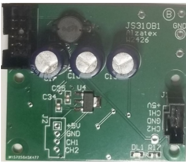
Microwave Input Amplifier and A2D PCB
