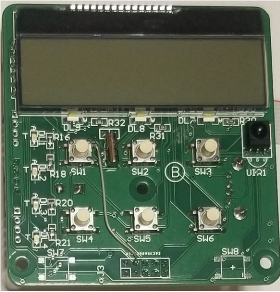
Main Microprocessor and Control PCB
