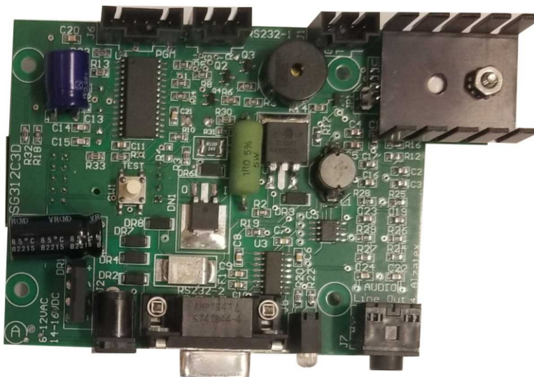
Power Supply and Battery Charger PCB
