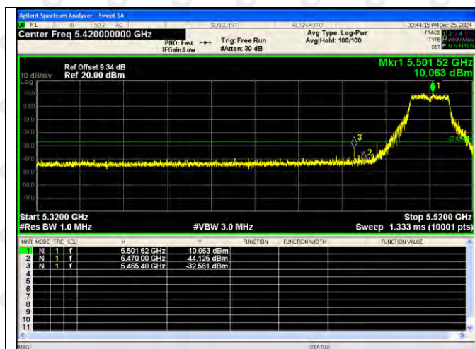
802.11ac(VH40)-5510
