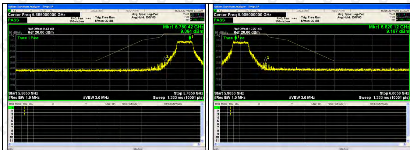
802.11ac(VH20)-5745
