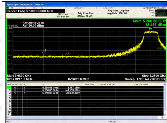
802.11n(HT40)-5270
