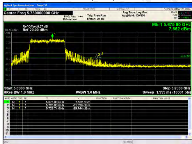
802.11ax(VH40)-5670
