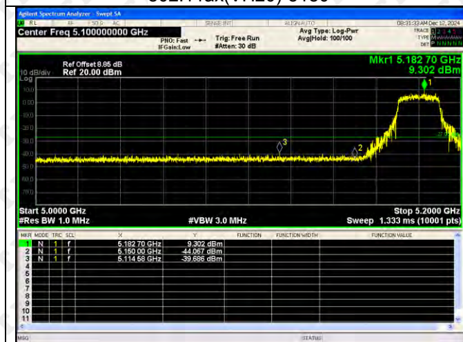
802.11ax(VH40)-5190
