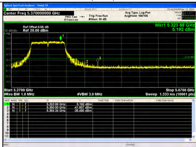
802.11ax(VH20)-5320
