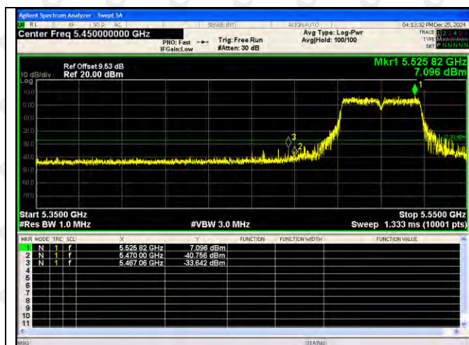
802.11ax(VH20)-5500
