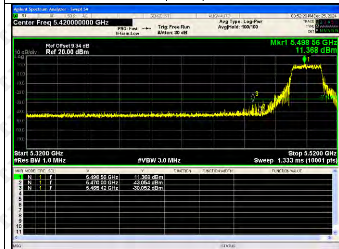
802.11ax(VH40)-5510
