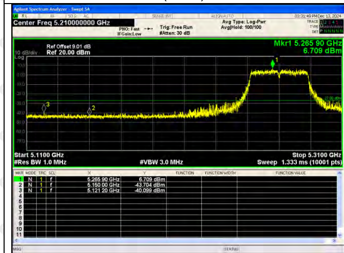
802.11ax(VH20)-5260
