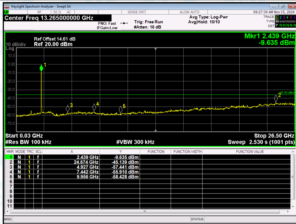
Tx. Spurious NVNT ax(VHT40) 2452MHz Ant1 Emission
