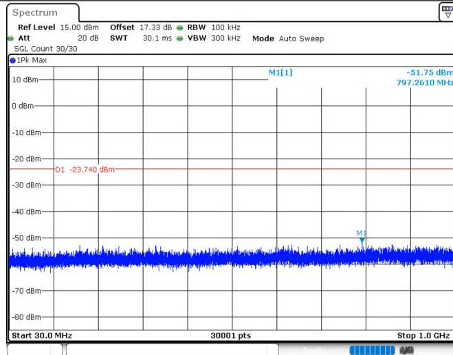
11N20SISO_Ant1_2412_30~1000
