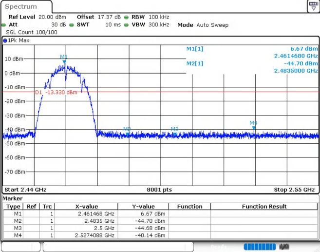
11B_Ant1_High_2462
