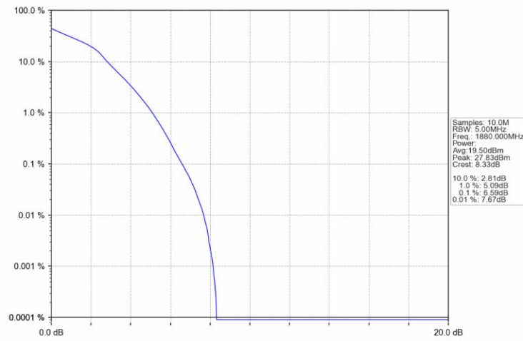
Band2_5MHz_16QAM_MCH_1880MHz_RB_25_0_NTNV
