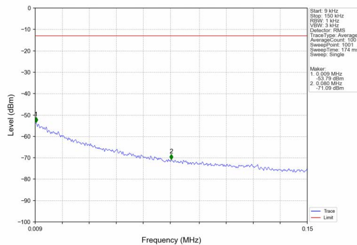
Band2_1.4MHz_16QAM_HCH_1909.3MHz_RB_1_0_NTNV
