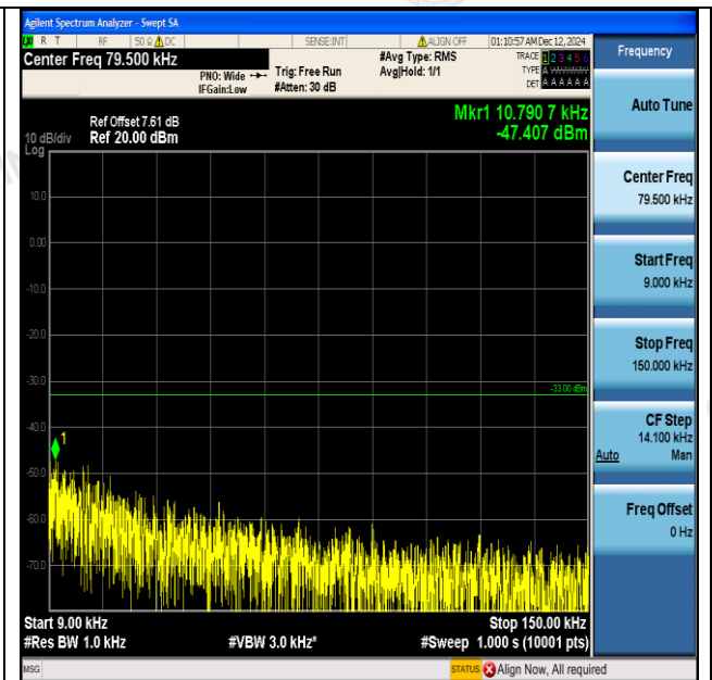
GPRS850-190-5-0.009~0.15MHz-PASS
