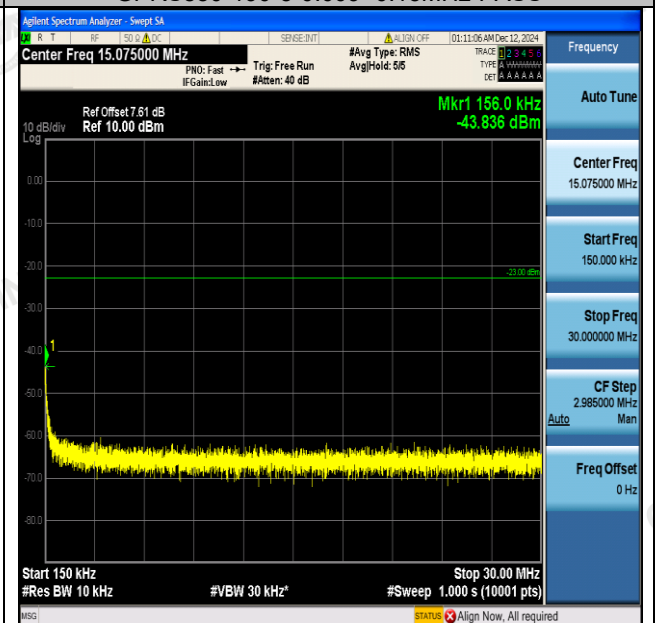
GPRS850-190-5-0.15~30MHz-PASS
