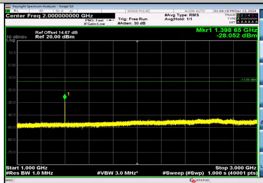
Band12_5MHz_16QAM_23035_1RB#0_1000~30 00_1000~3000
