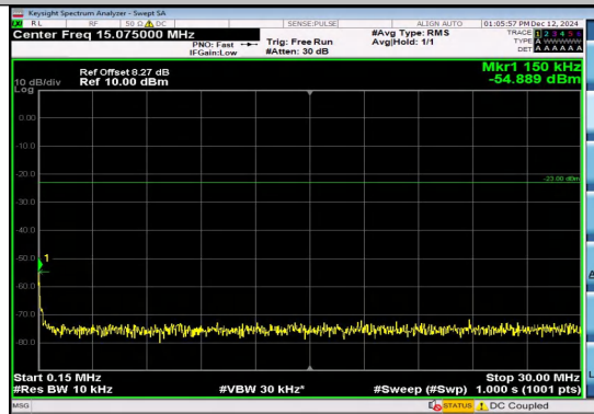
Band12_5MHz_16QAM_23035_1RB#0_0.15~30 _0.15~30
