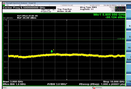
Band12_5MHz_16QAM_23035_1RB#0_3000~100 00_3000~10000
