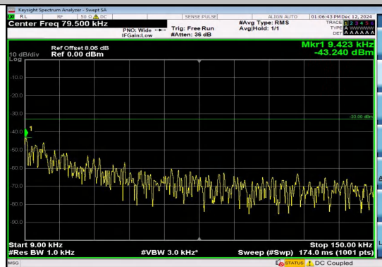
Band12_5MHz_QPSK_23095_1RB#0_0.009~0.1 5_0.009~0.15
