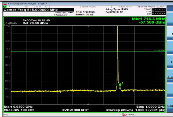
Band12_5MHz_16QAM_23035_1RB#0_30~1000 30~1000
