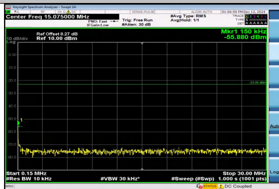
Band12_5MHz_QPSK_23095_1RB#0_0.15~30_0. 15~30
