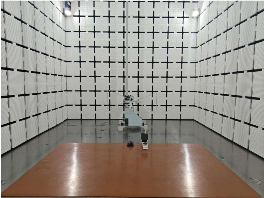
Radiated Emission Test View 4(Watch)
