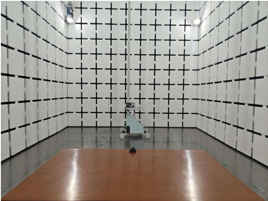
Radiated Emission Test View 3(Watch)
