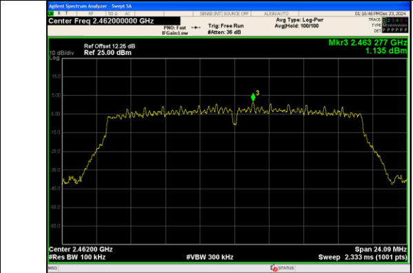
In-Band Reference Level IEEE 802.11n_Channel 11_20MHz_Antenna 0
