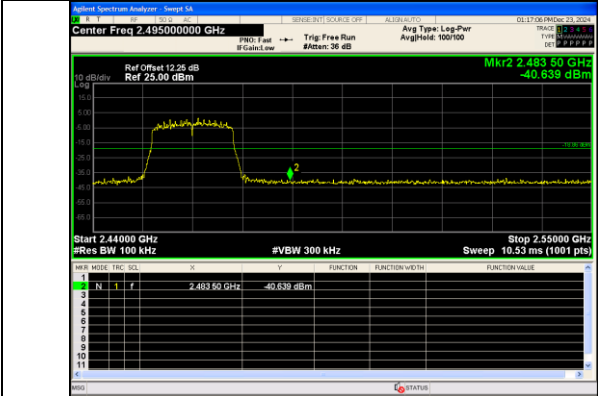
Out Of Band Emission IEEE 802.11n_Channel 11_20MHz_Antenna 0
