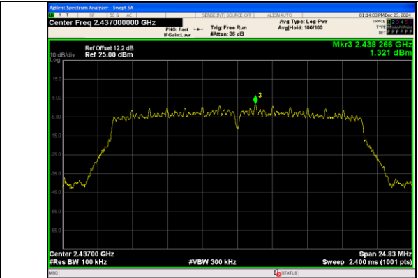
In-Band Reference Level IEEE 802.11n_Channel 6_20MHz_Antenna 0
