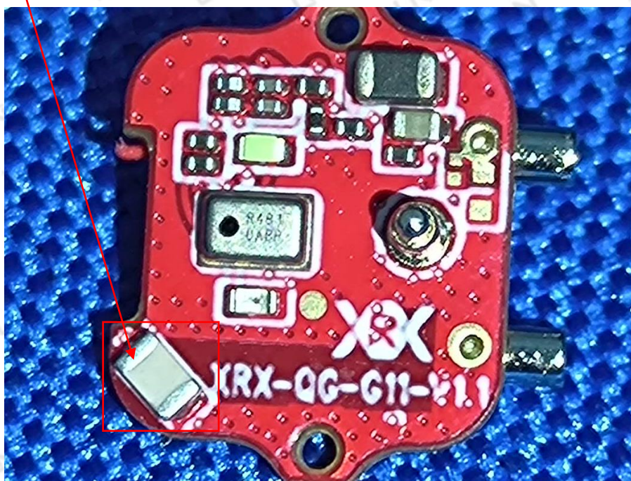
Chip Antenna
