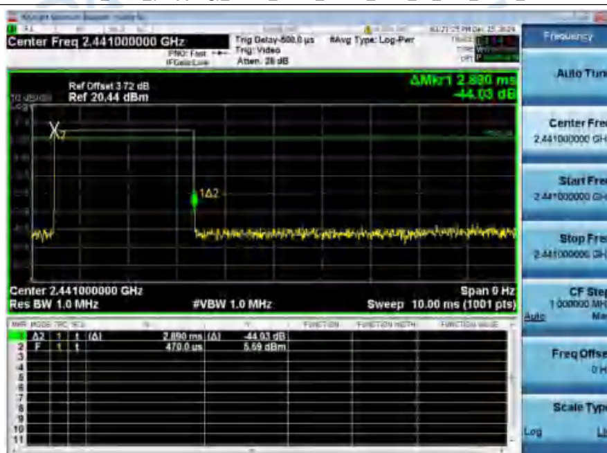
Dwell_Time_(Hopping)_NVNT_ANT1_1-DH5_2441_00_Accumulated
