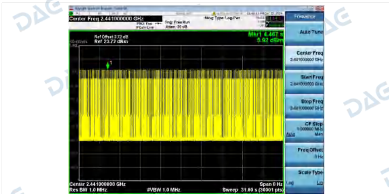
Dwell_Time_(Hopping)_NVNT_ANT1_3-DH3_2441_00_One_Burst_Time
