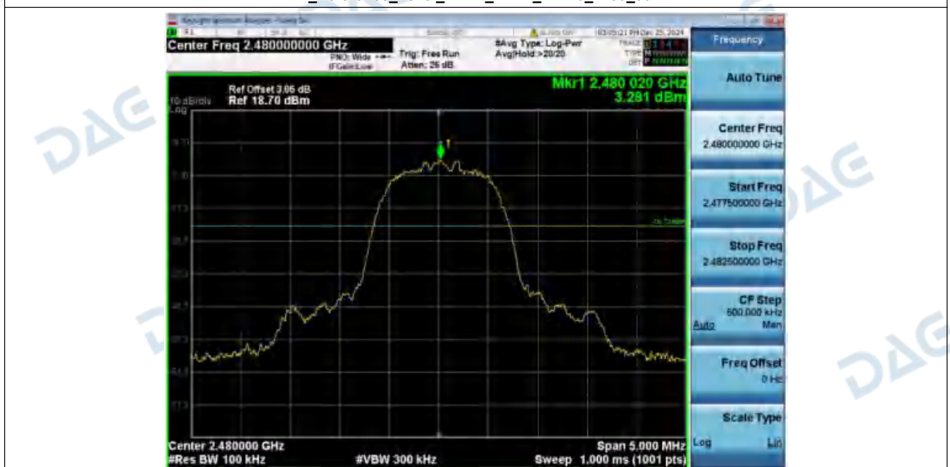
2_Bandedge_NVNT_ANT1_2-DH5_2480_00
