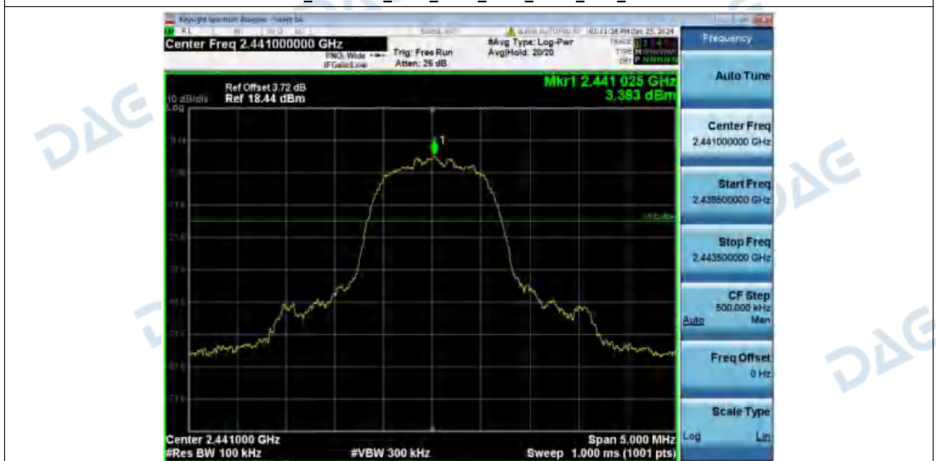
2_Spurious_Emissions_NVNT_ANT1_3-DH5_2441_00
