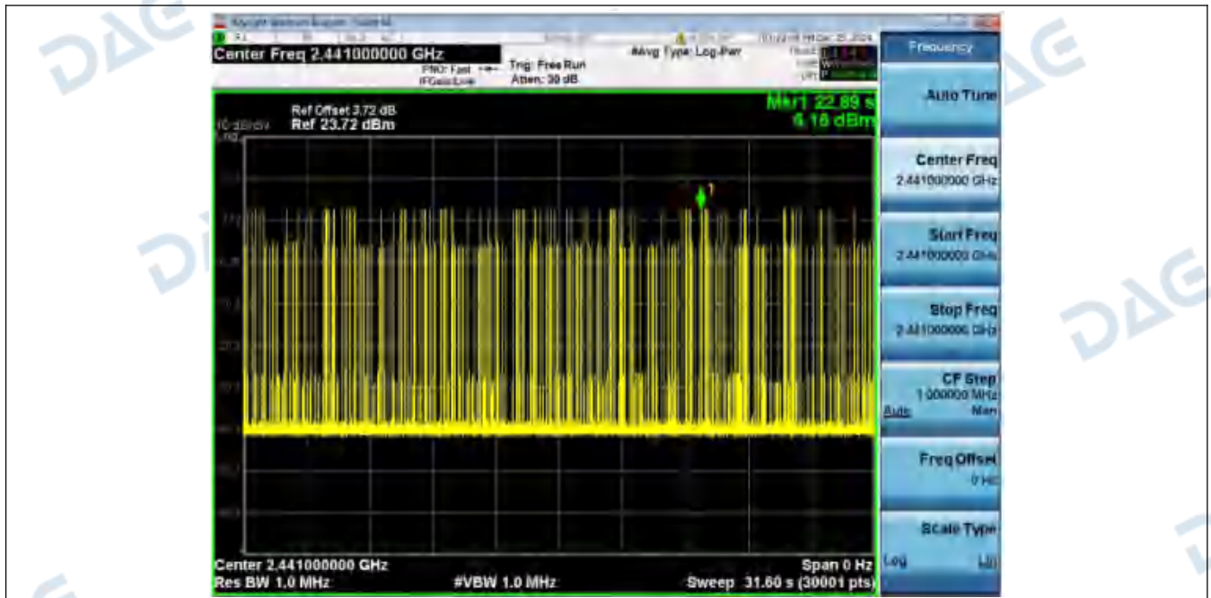
Dwell_Time_(Hopping)_NVNT_ANT1_2-DH5_2441_00_One_Burst_Time
