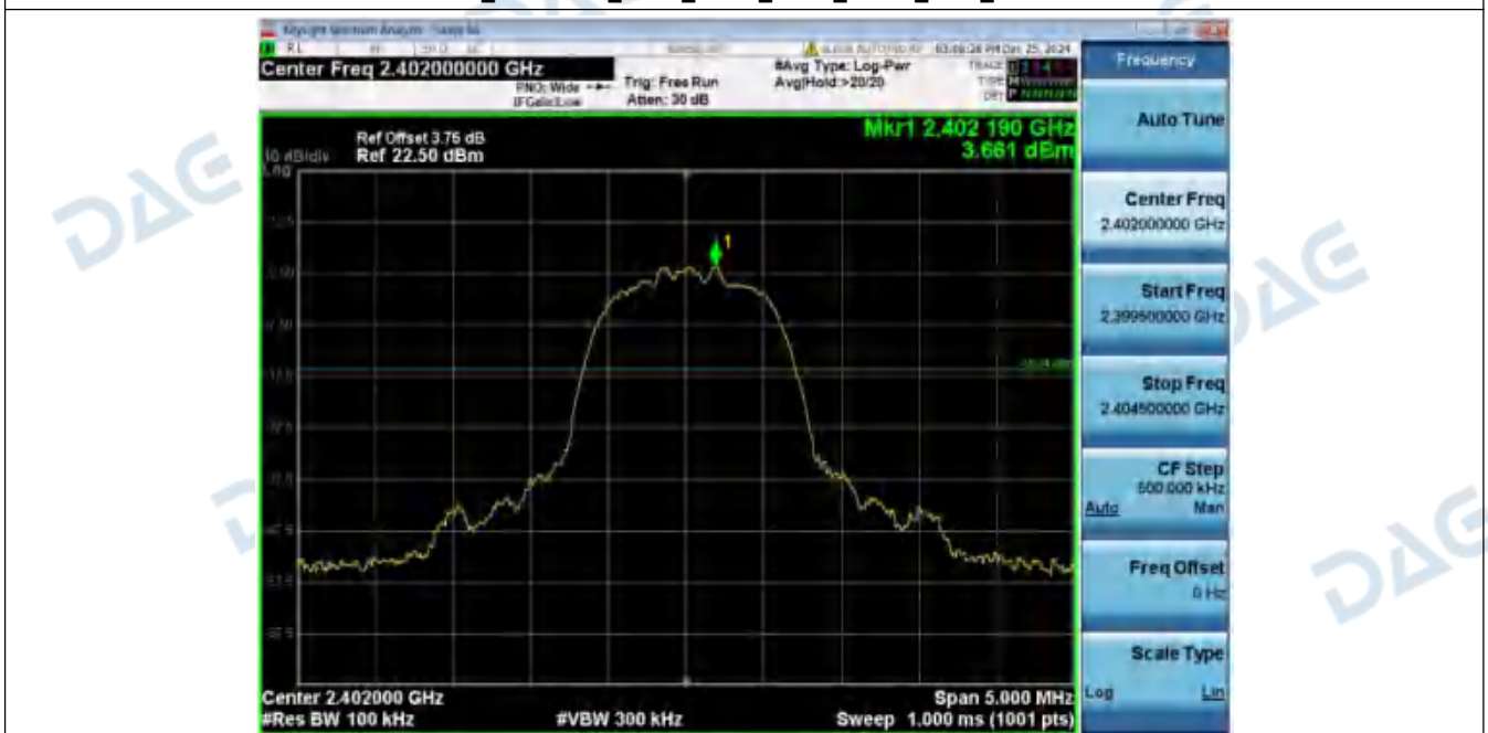
2_Bandedge_NVNT_ANT1_3-DH5_2402_00
