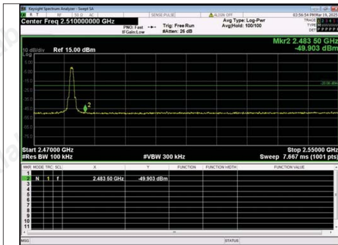
Out Of Band Emission BLE 1M_Channel 39
