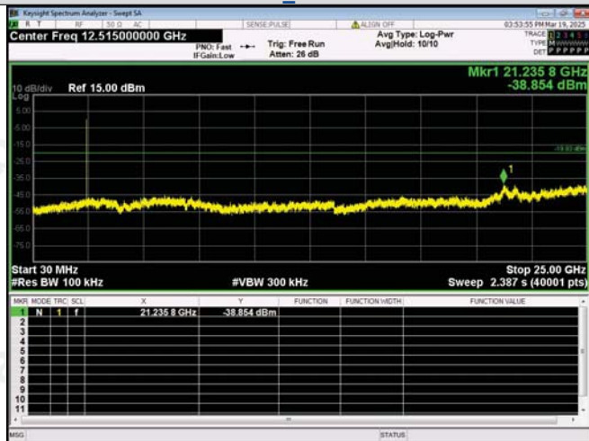
30.0 MHz - 25000.0 MHz BLE 1M_Channel 19
