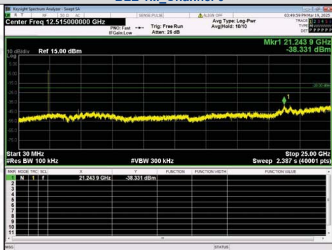
30.0 MHz - 25000.0 MHz BLE 1M_Channel 0
