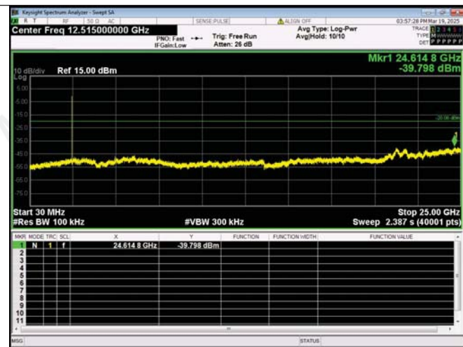
30.0 MHz - 25000.0 MHz BLE 1M_Channel 39
