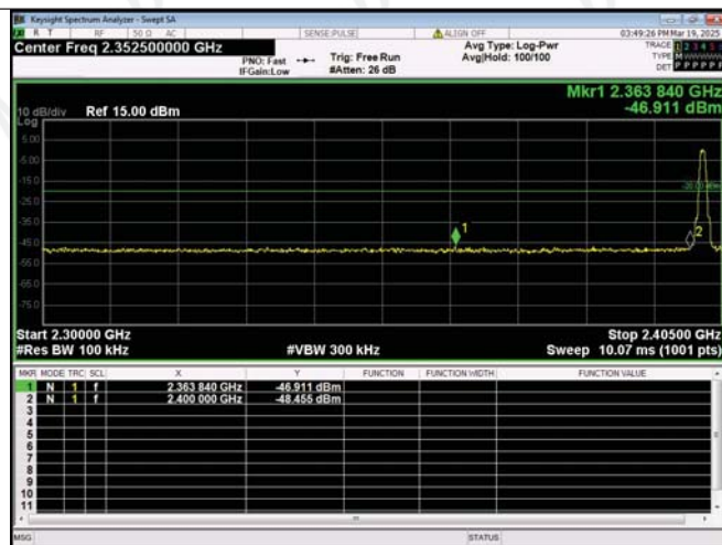
Out Of Band Emission BLE 1M_Channel 0
