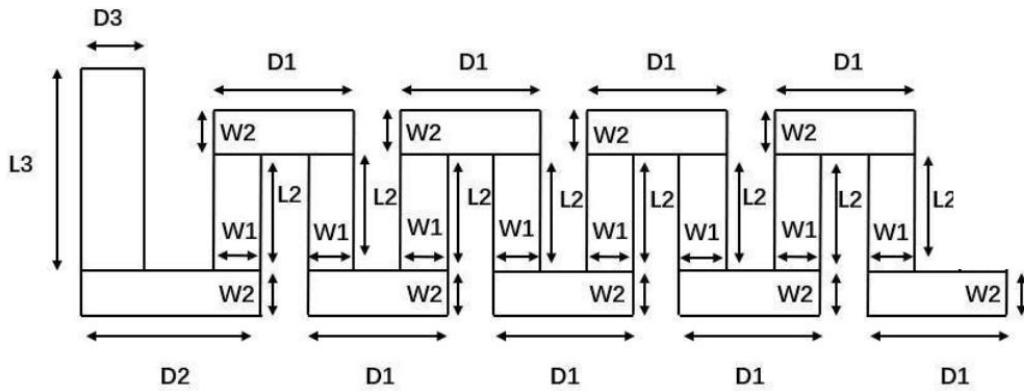
Antenna Dimensions
