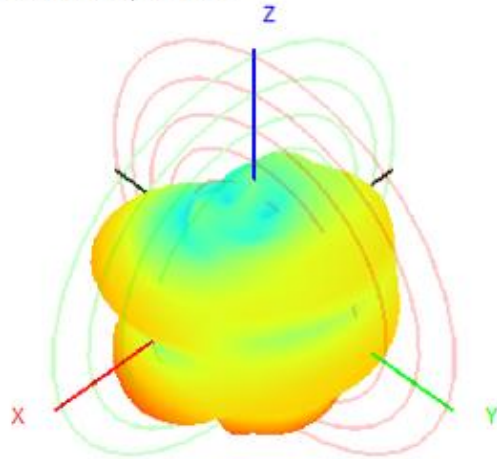
433.0MHz H+V, Eff: 4.8%
