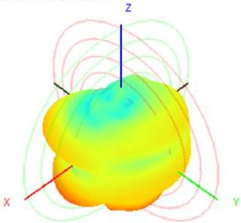
434.0MHz H+V, Eff: 4.7%
