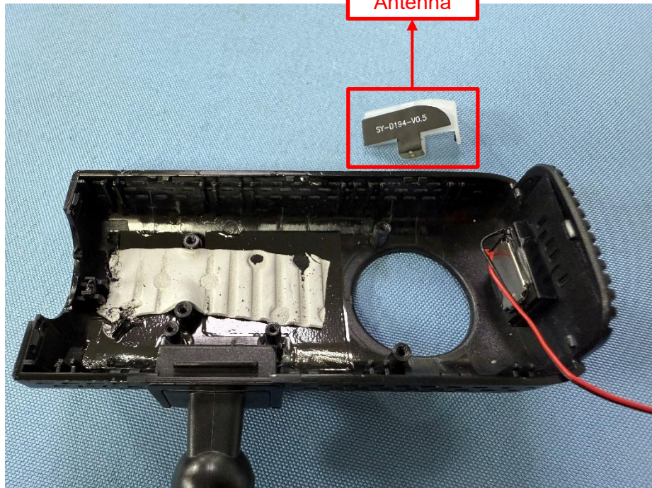
WIFI Antenna
