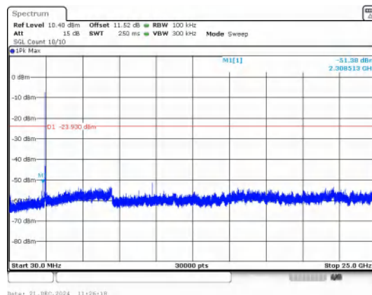
30.0 MHz - 25000.0 MHz \pi/4 QPSK_2-DH5_Channel 39
