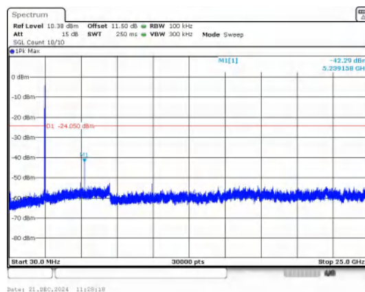
30.0 MHz - 25000.0 MHz \pi/4 QPSK_2-DH5_Channel 78
