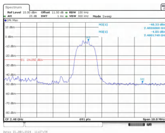
Out Of Band Emission \pi/4 QPSK_2-DH5_Channel 78
