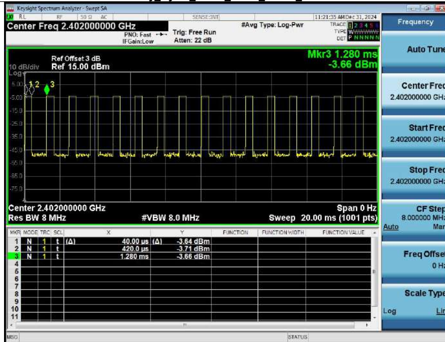
Duty_Cycle_NVNT_ANT1_1-DH1_2402
