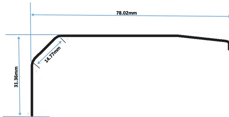
Antenna size diagram:
