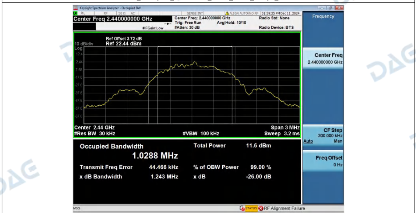
99%_Occupied_Bandwidth_NVNT_ANT1_1Mbps_2440
