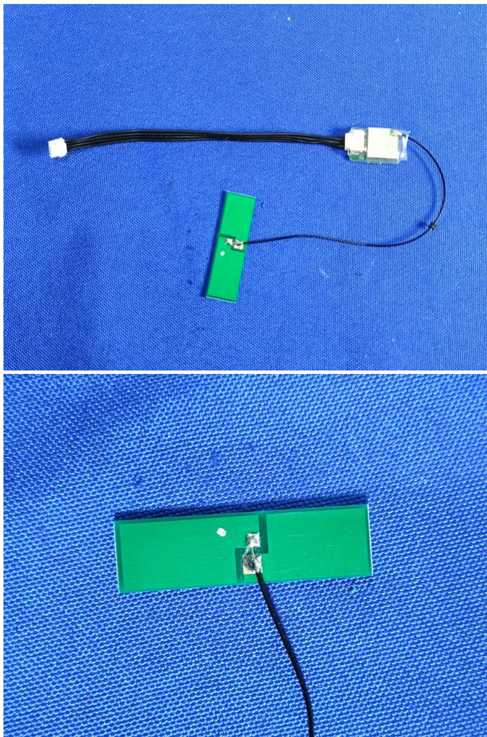
Inside View-WIFI
