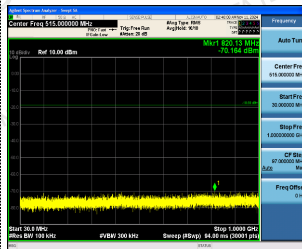
30MHz-1GHz
