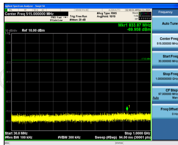
30MHz-1GHz
