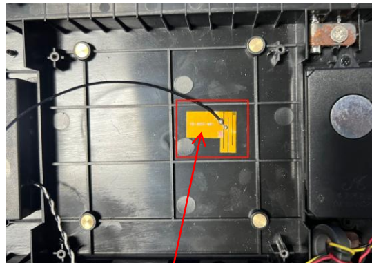
FPC Antenna
