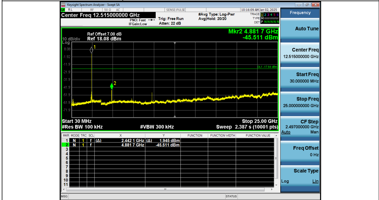
2 Spurious Emissions NVNT ANT1 2-DH1 2441_00
