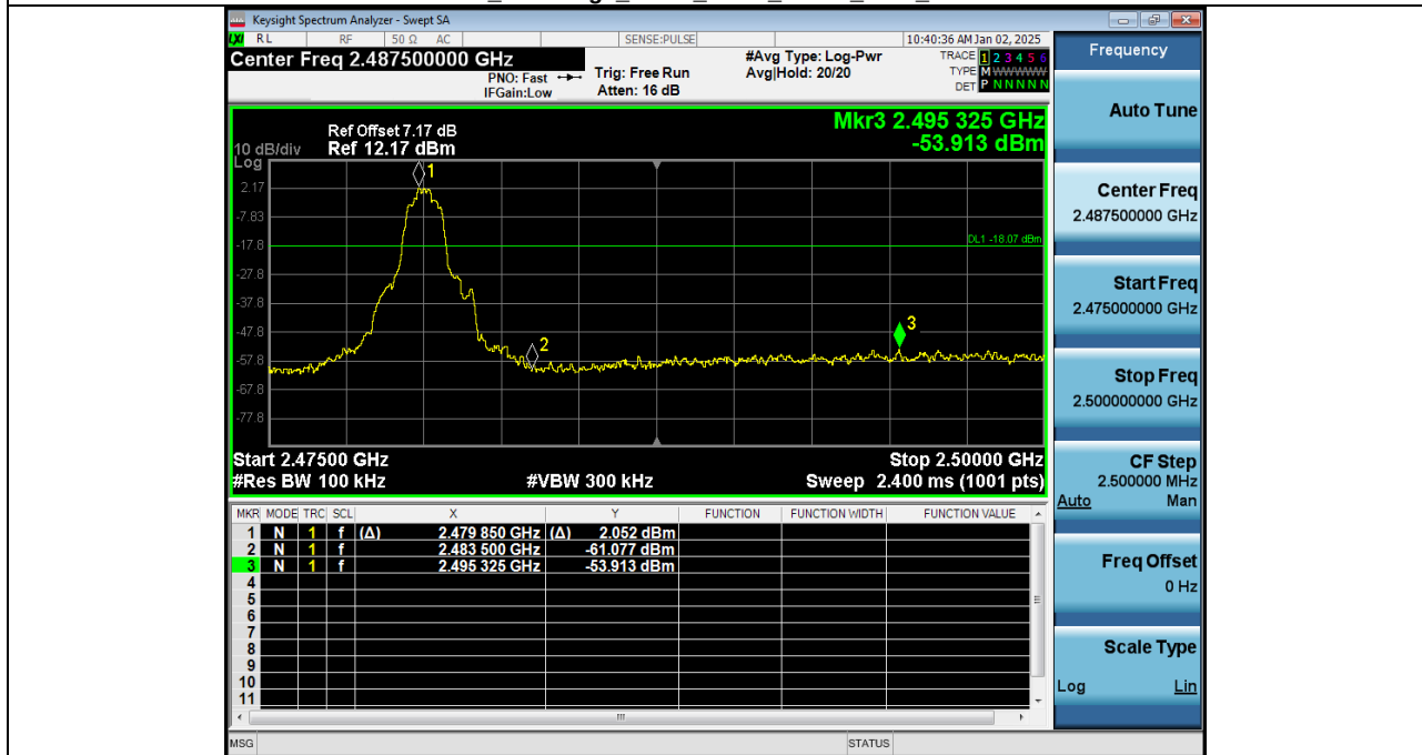
2_Bandedge_NVNT_ANT1_3-DH1_2480_00
