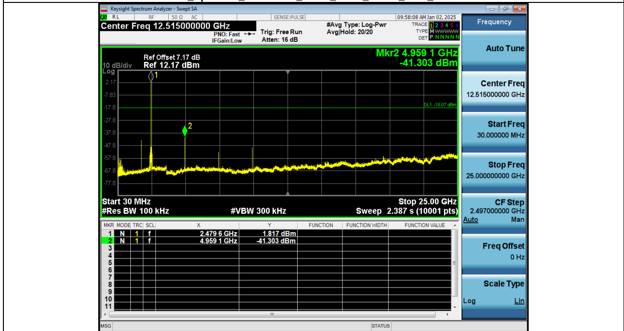
2 Spurious Emissions NVNT_ANT1_1-DH1_2480_00
