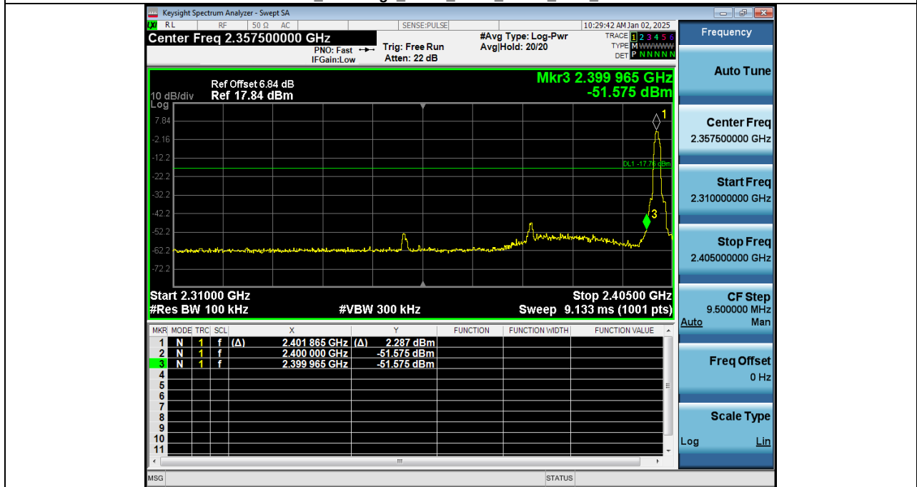
2_Bandedge_NVNT_ANT1_3-DH1_2402_00
