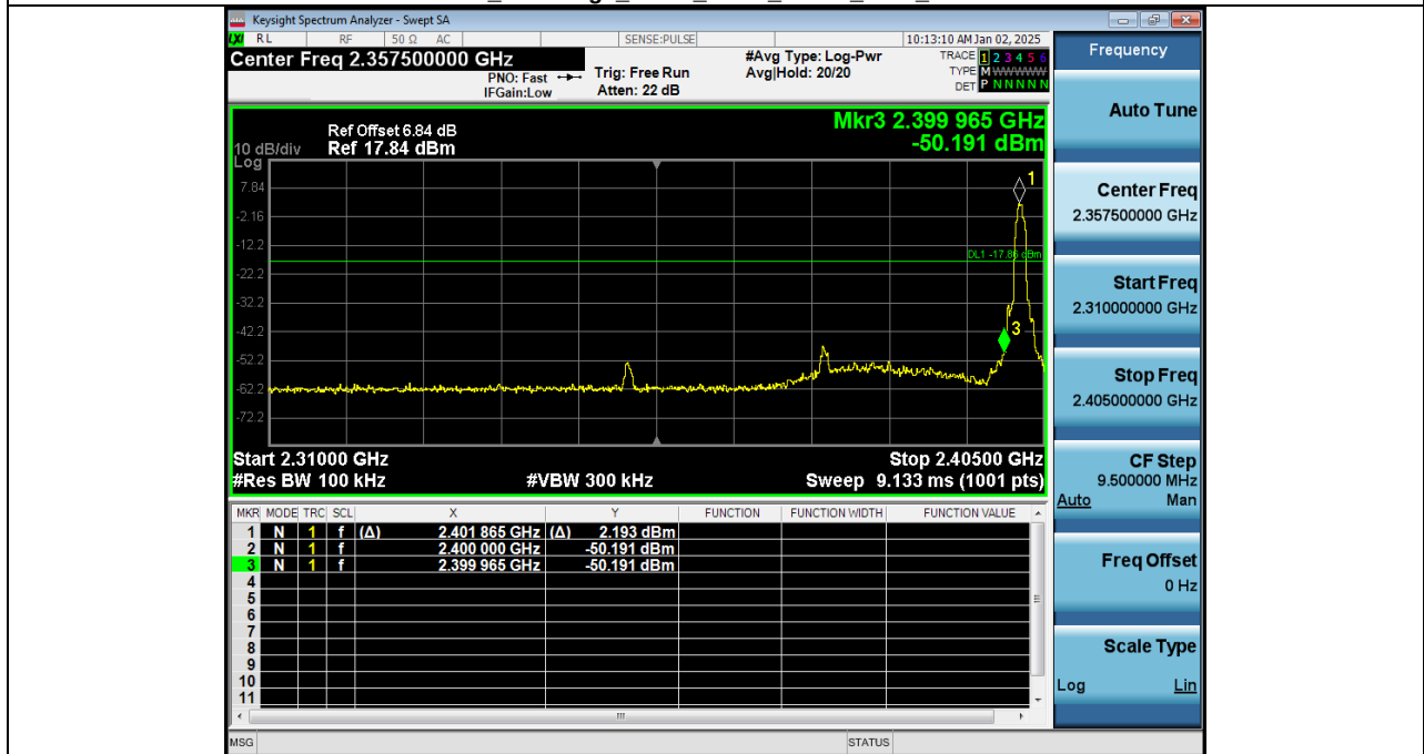
2_Bandedge_NVNT_ANT1_2-DH1_2402_00
