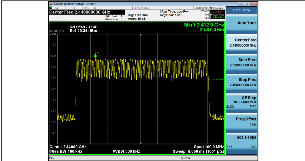
2_Band_Edge_(Hopping)_NVNT_ANT1_1-DH1_Hopping
