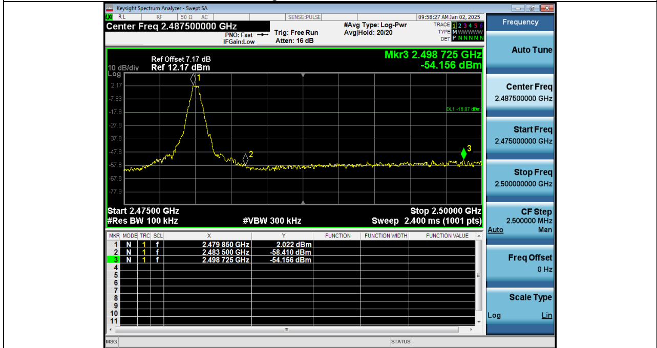
2_Bandedge_NVNT_ANT1_1-DH1_2480_00
