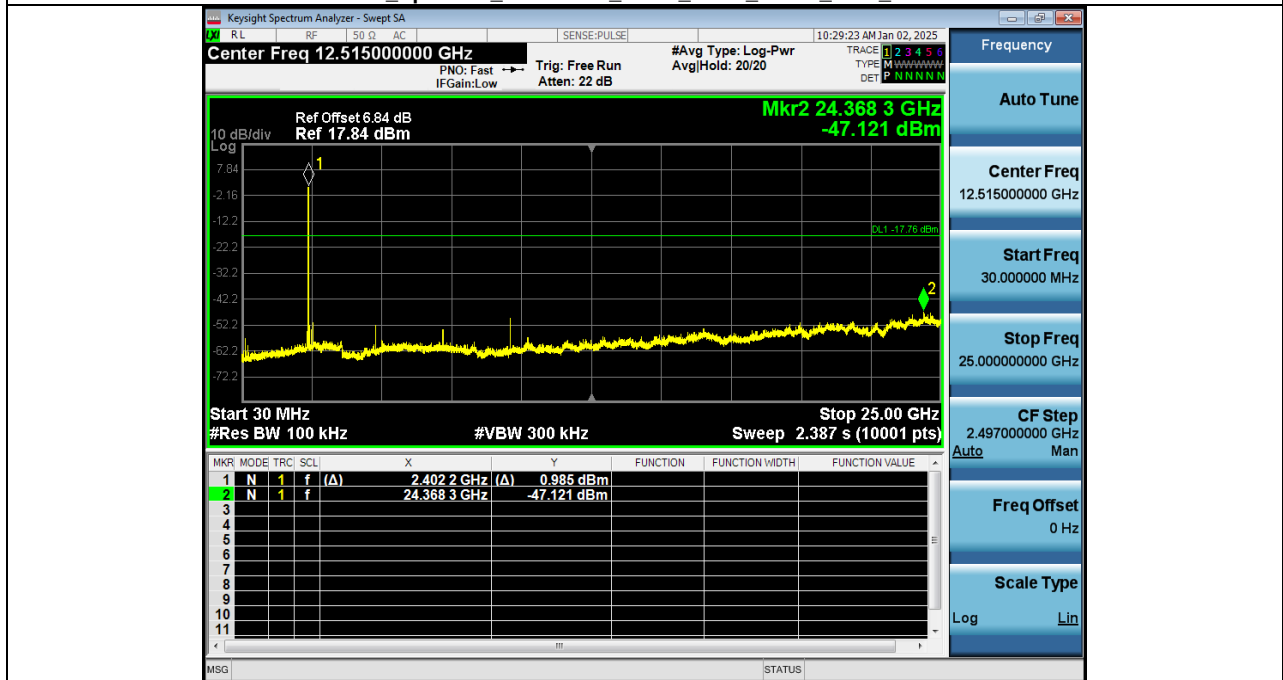
2 Spurious Emissions NVNT_ANT1_3-DH1_2402_00
