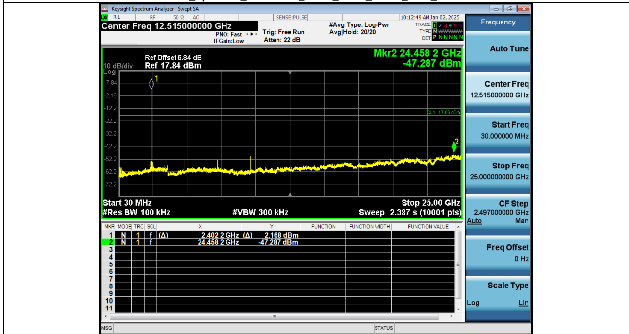
2 Spurious Emissions_NVNT_ANT1_2-DH1_2402_00
