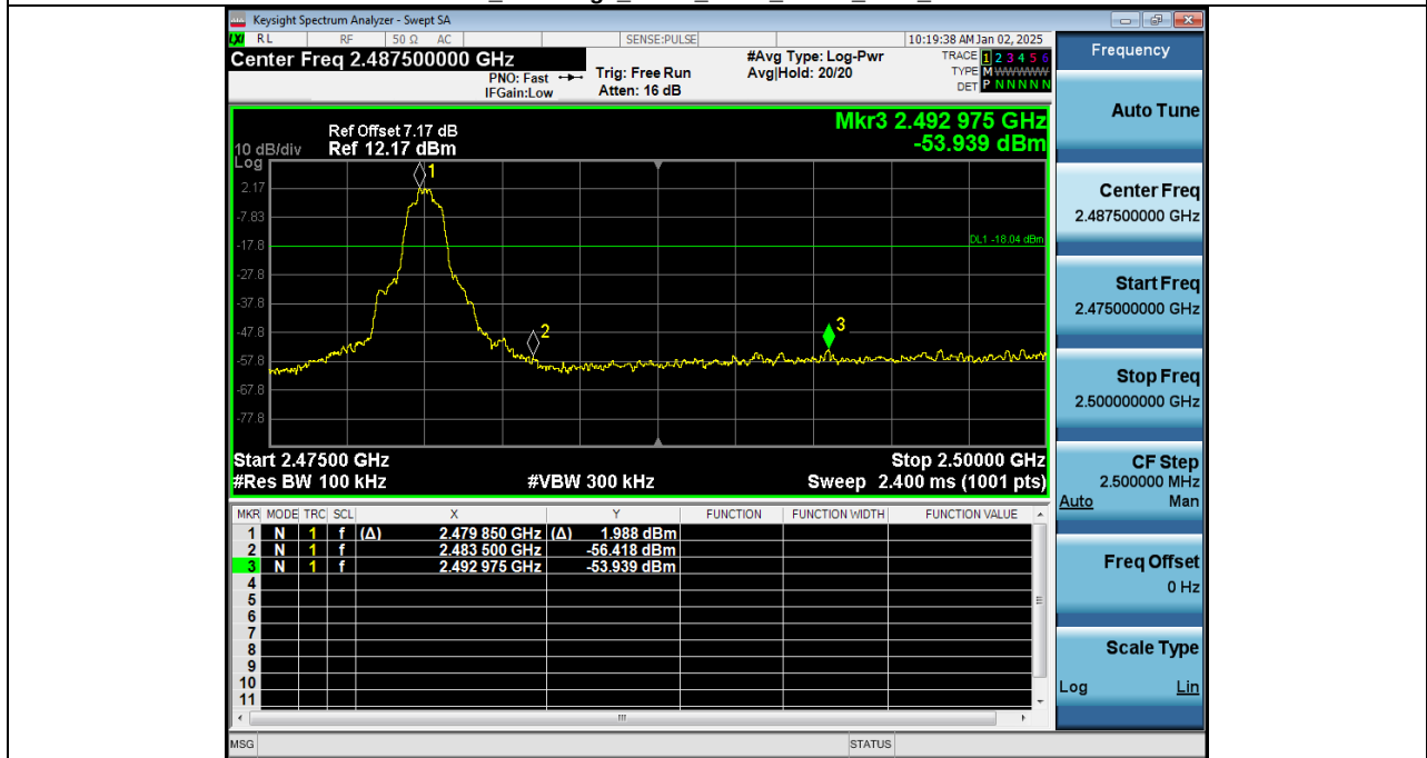
2_Bandedge_NVNT_ANT1_2-DH1_2480_00
