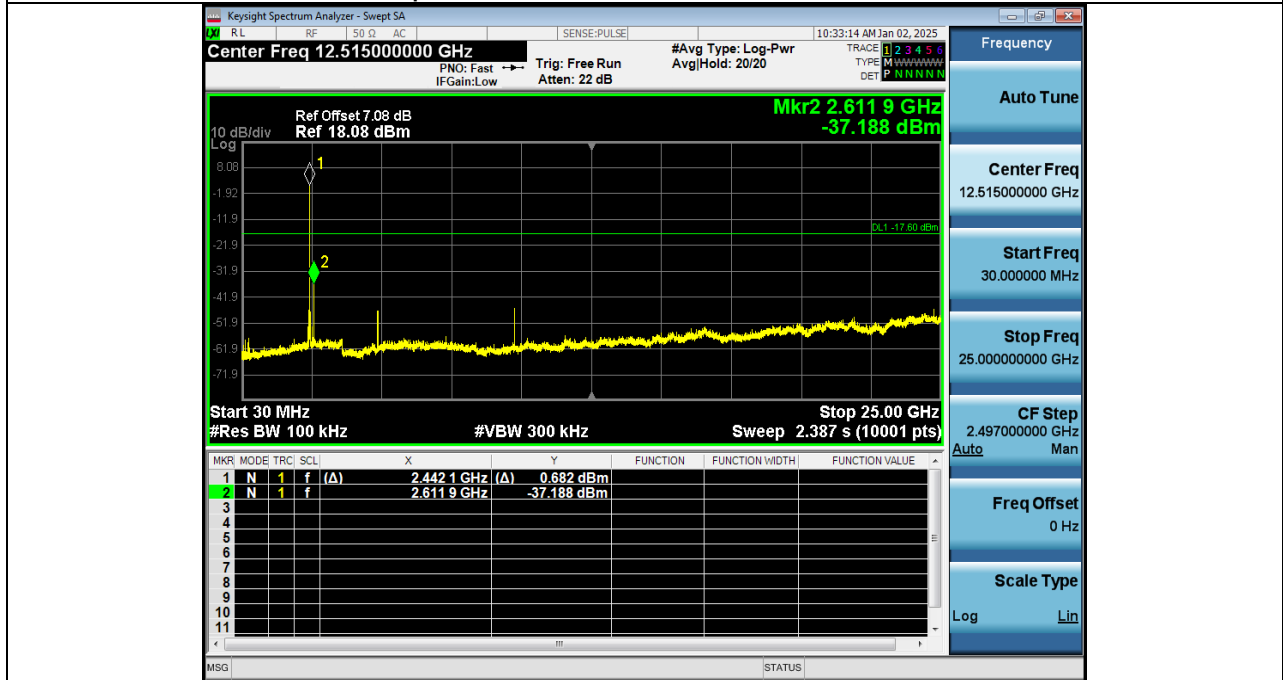
2 Spurious Emissions NVNT_ANT1_3-DH1_2441_00
