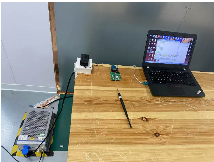
Conducted Emission - 1
