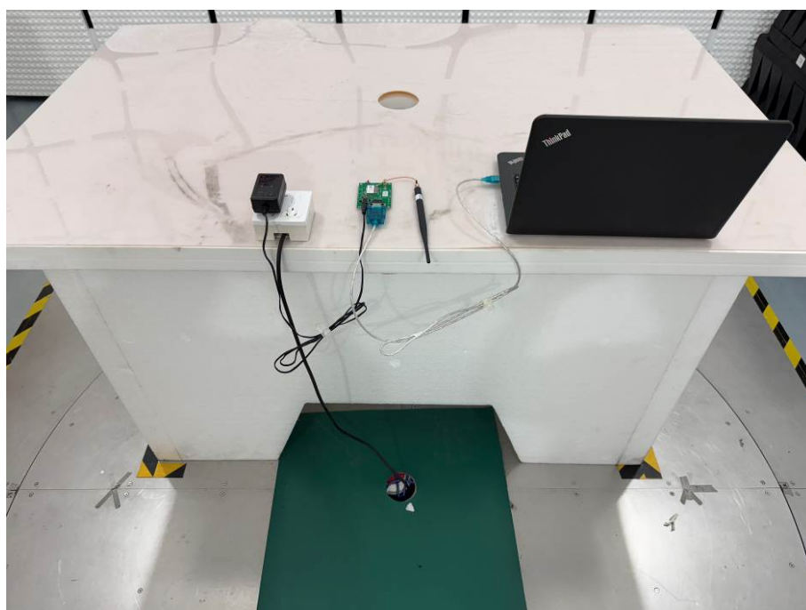
Below 1GHz - 2
